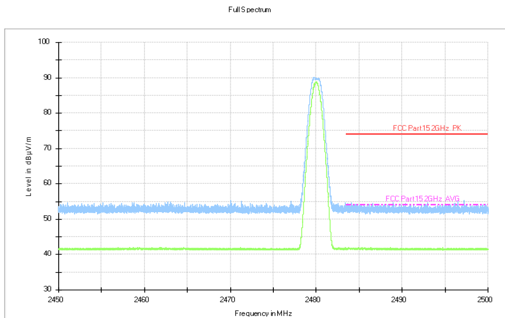
Fig.4. Frequency Band Edges: GFSK, 2480 MHz, Hopping Off, 2.45 GHz - 2.50GHz
