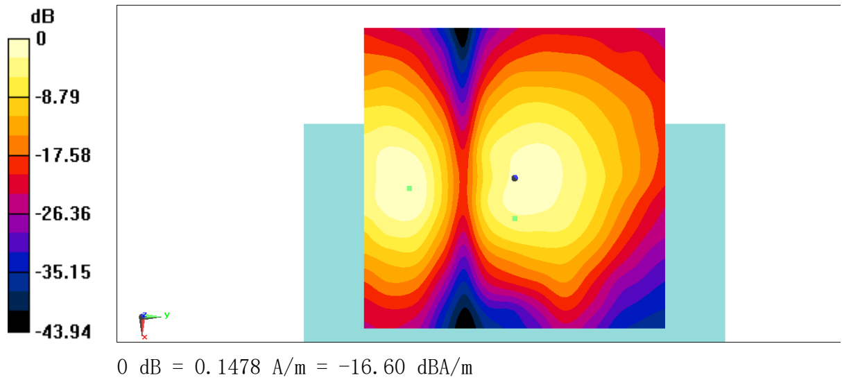
Fig B3 T-Coil LTE B2
