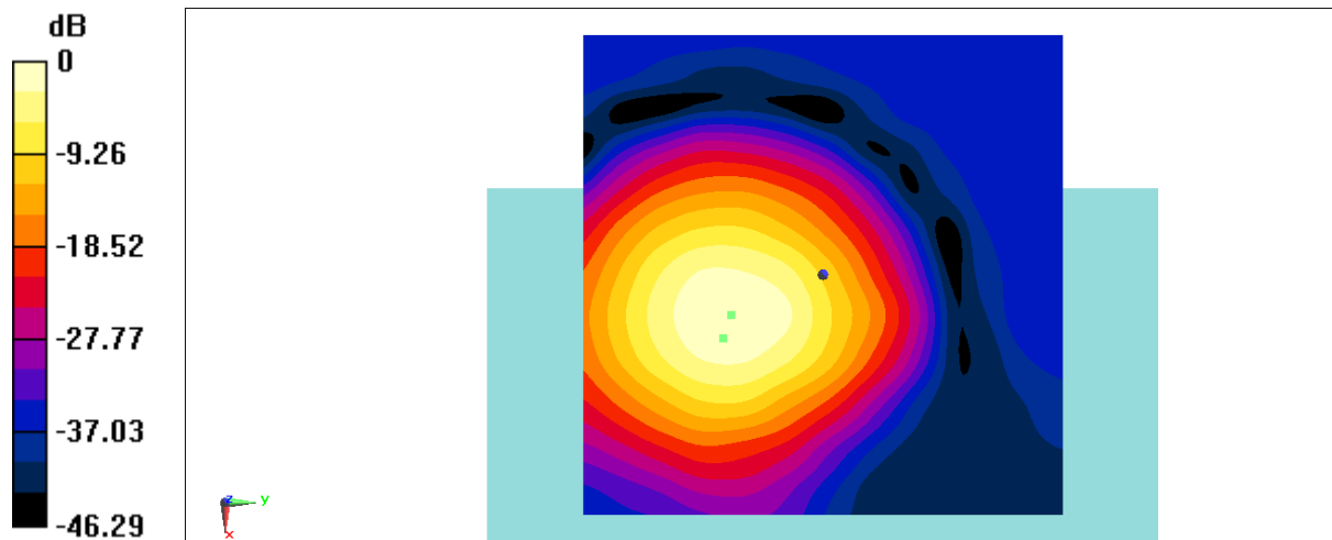
Fig B4 T-Coil LTEB2
