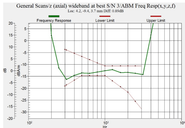
Figure C.2 Frequency Response of LTEB2 – OTT VoIP
