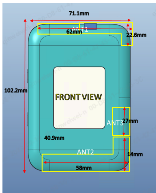
Picture 18: Antenna Location
