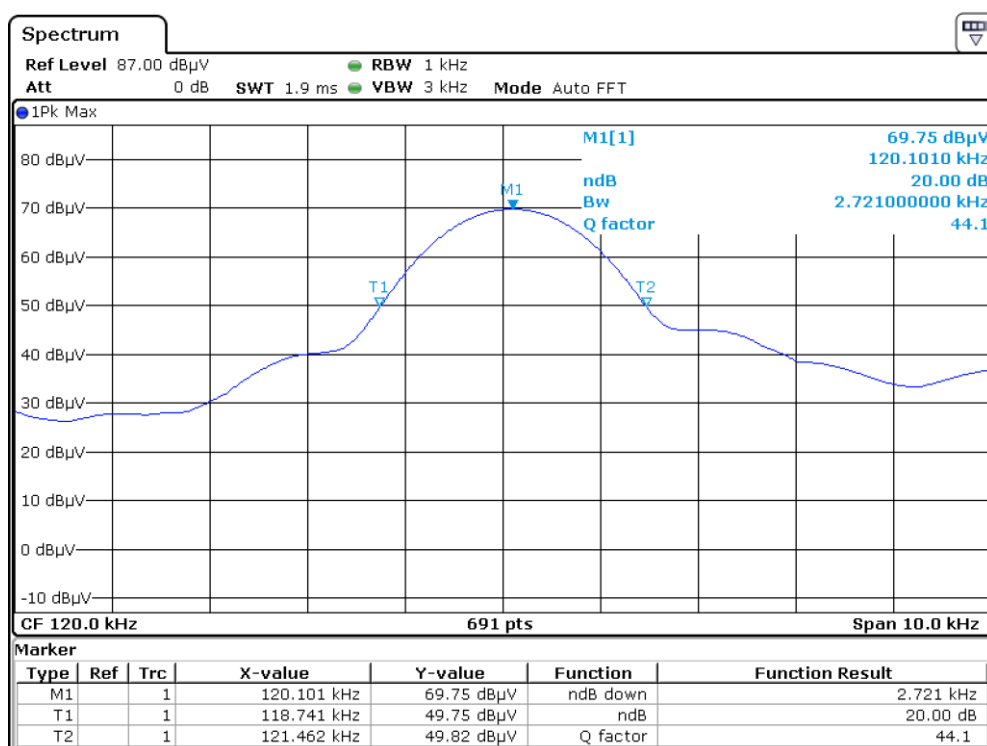
Output A
