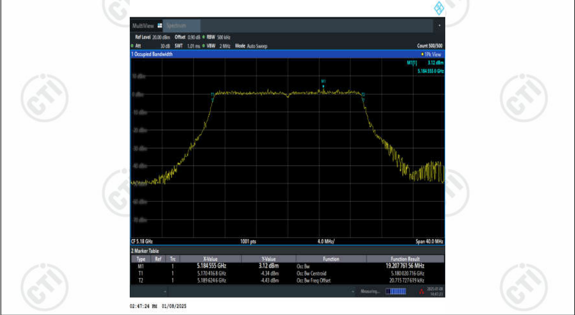
11AX20SISO-Ant2-5180
