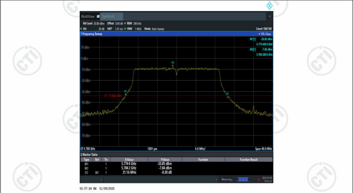
11AC20SISO-Ant2-5785
