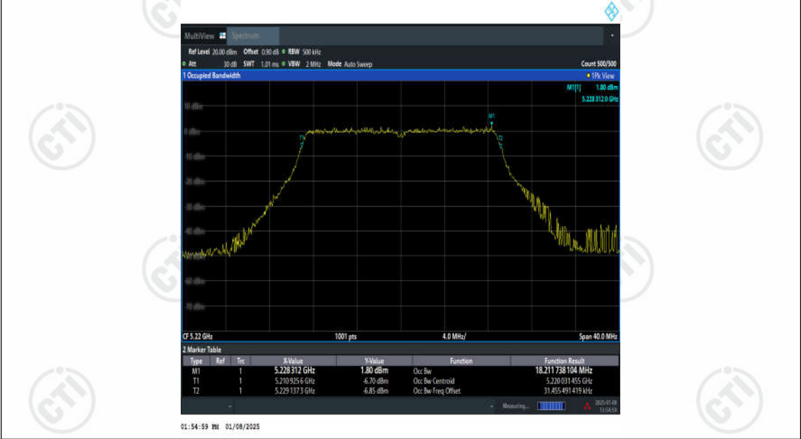
11AC20SISO-Ant2-5220
