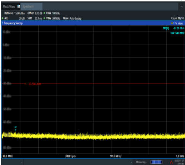
11N20SISO-Ant1-2412-30~1000-PASS
