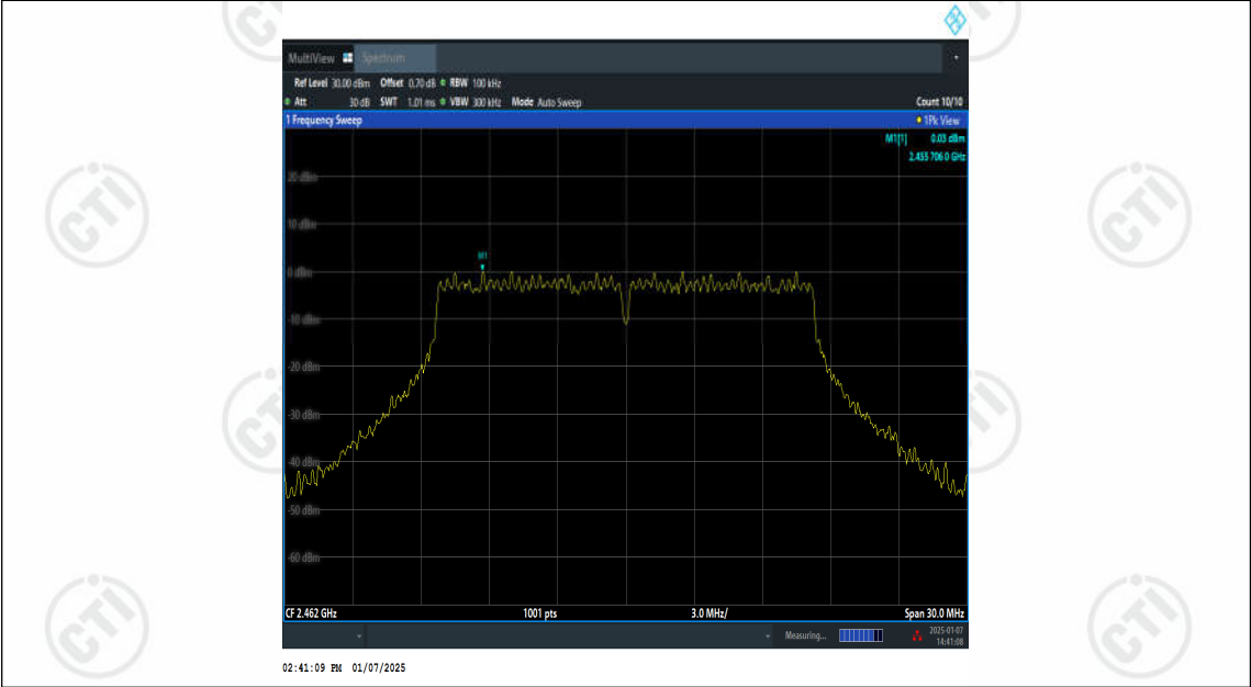
11G-Ant2-2462-0~Reference-PASS
