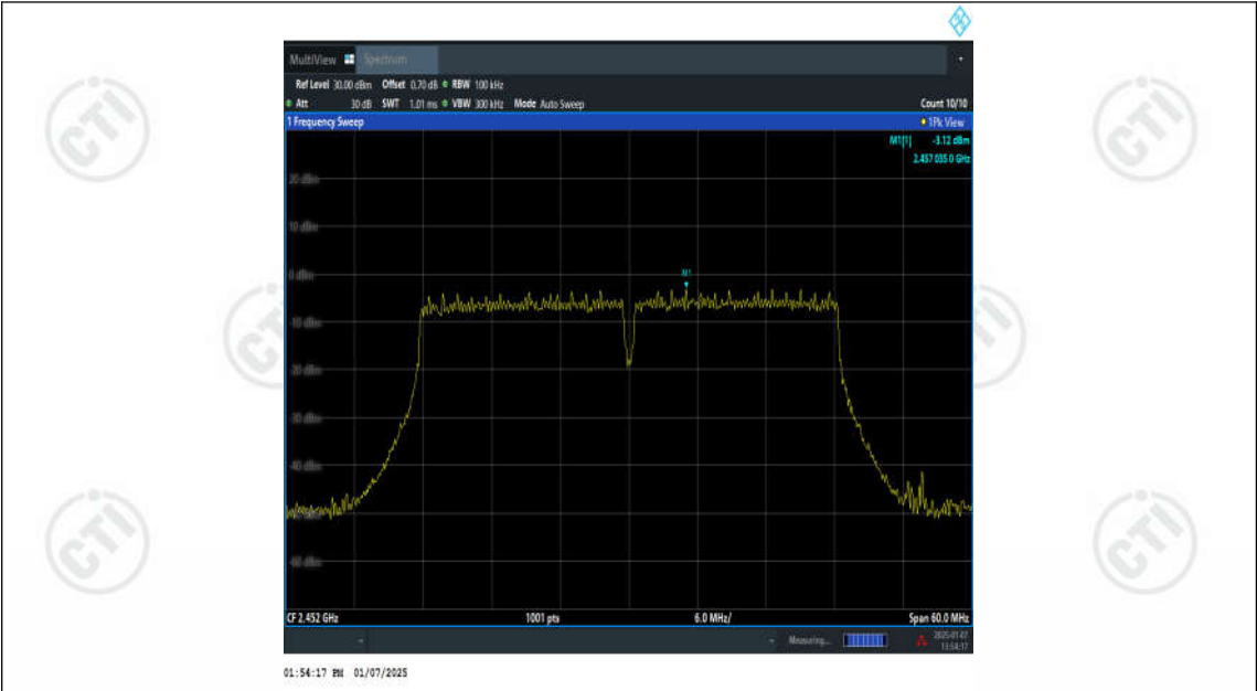
11N40SISO-Ant1-2452-0~Reference-PASS
