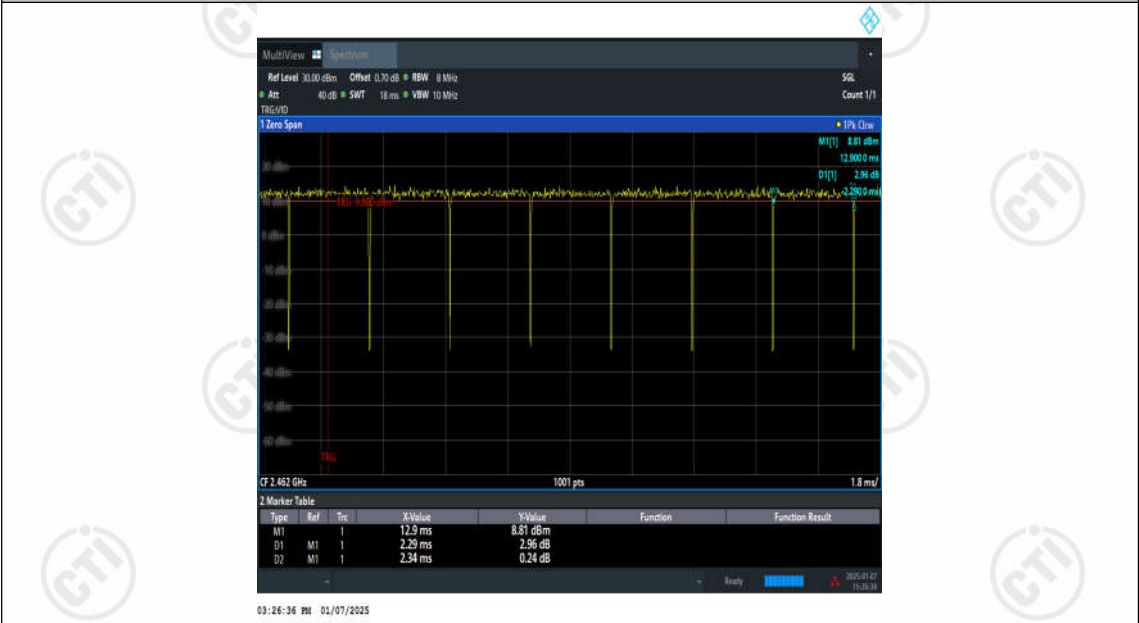
NTNV-11AX20MIMO-Ant2-2462
