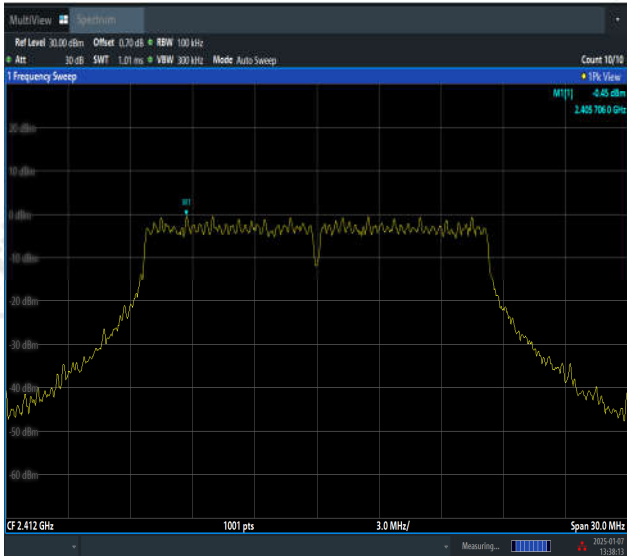
11G-Ant1-2412-0~Reference-PASS
