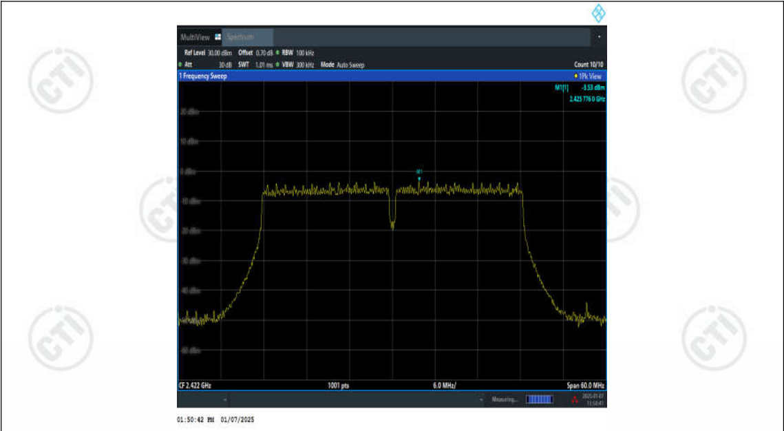
11N40SISO-Ant1-2422-0~Reference-PASS
