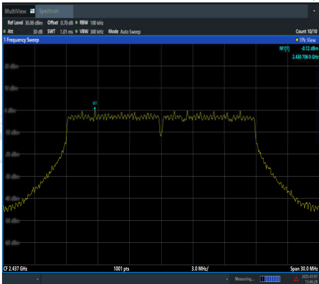
11N20SISO-Ant1-2437-0~Reference-PASS
