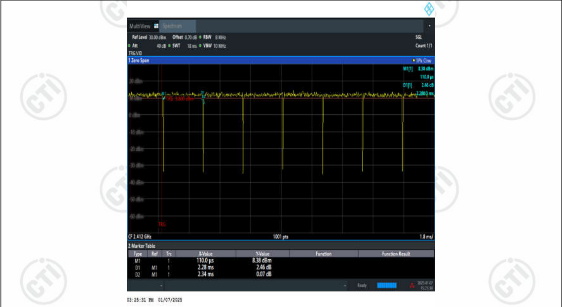
NTNV-11AX20MIMO-Ant2-2412
