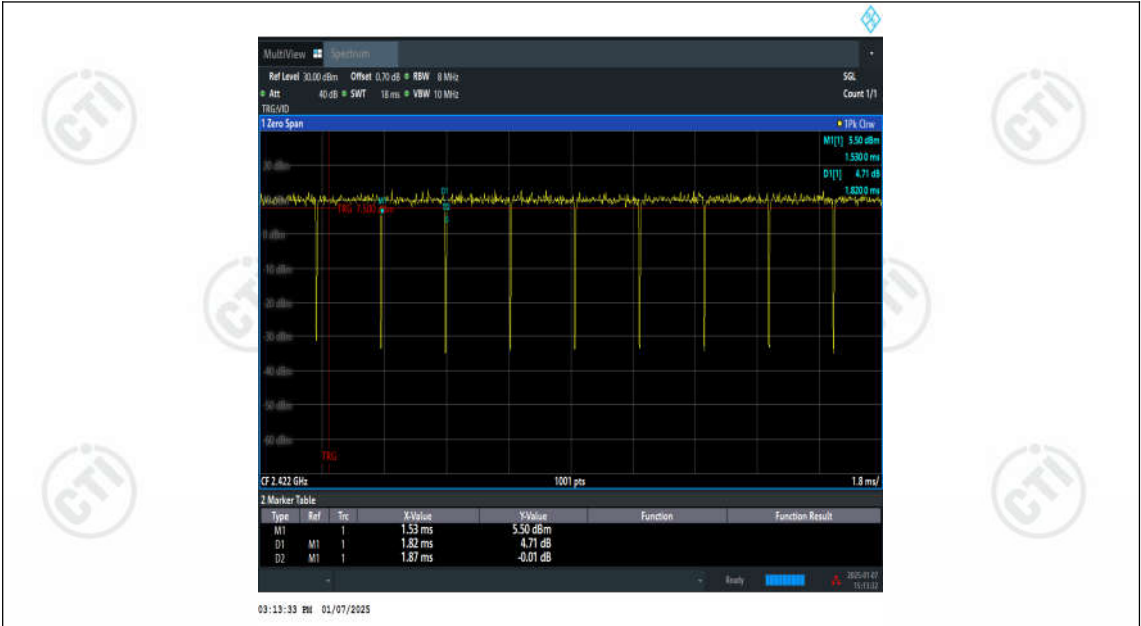
NTNV-11N40MIMO-Ant1-2422
