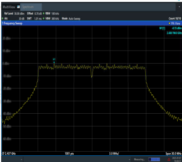
11N20SISO-Ant2-2437-0~Reference-PASS
