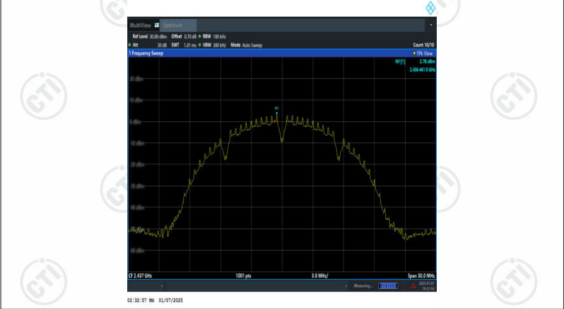
11B-Ant2-2437-0~Reference-PASS
