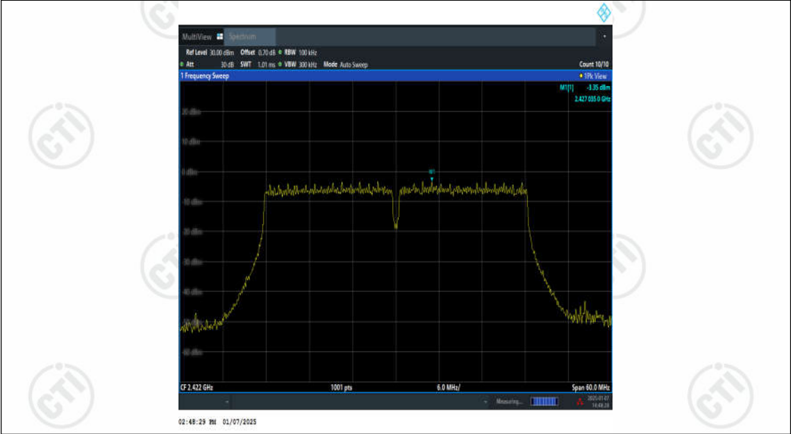
11N40SISO-Ant2-2422-0~Reference-PASS
