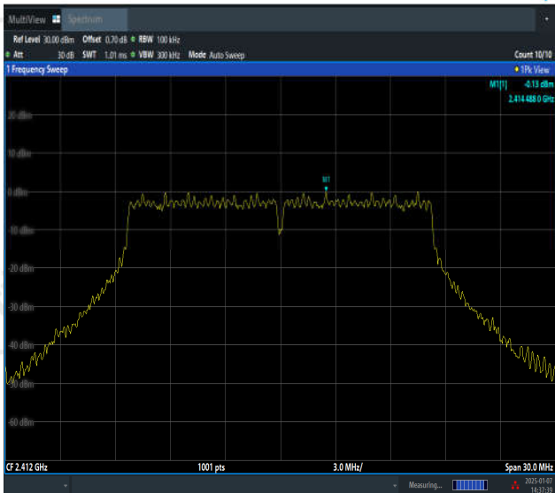
11G-Ant2-2412-0~Reference-PASS
