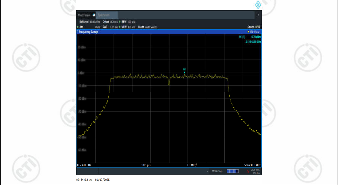
11AX20SISO-Ant2-2412-0~Reference-PASS
