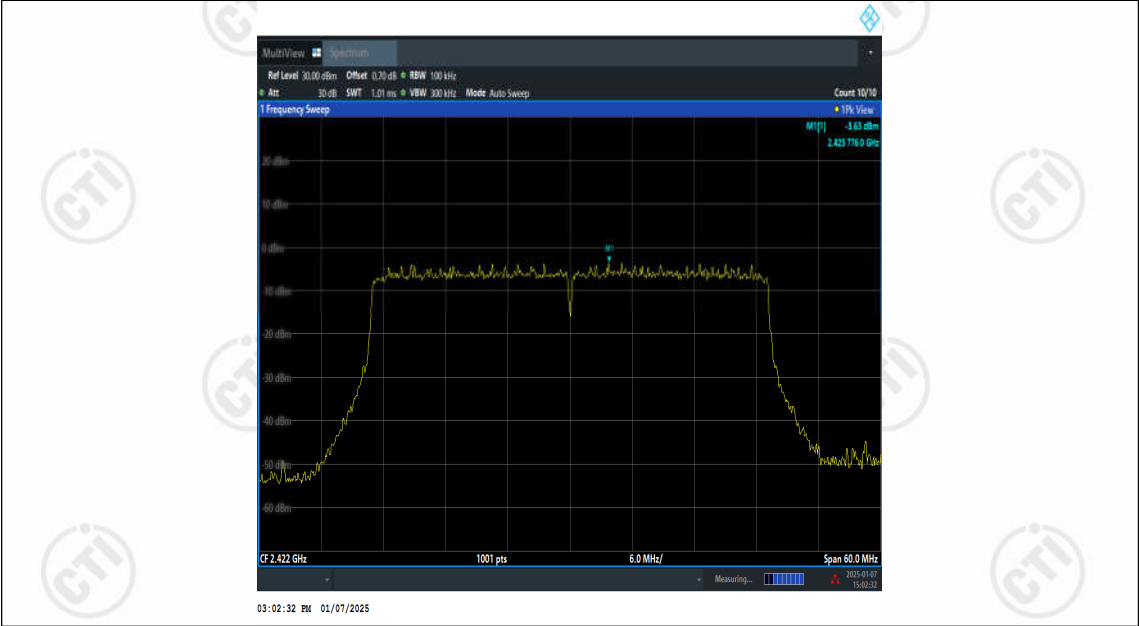
11AX40SISO-Ant2-2422-0~Reference-PASS
