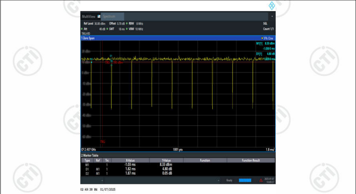
NTNV-11N40SISO-Ant2-2437
