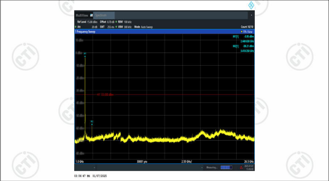
11AX40SISO-Ant2-2452-1000~26500-PASS
