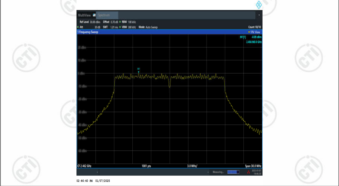
11N20SISO-Ant2-2462-0~Reference-PASS
