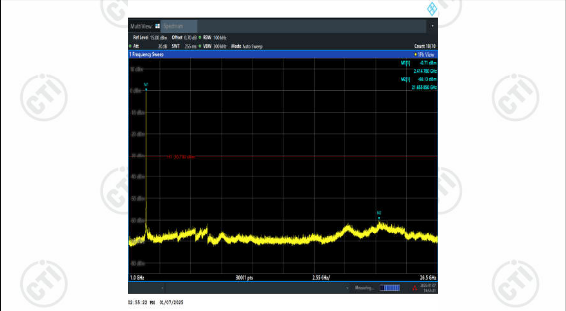
11AX20SISO-Ant2-2412-1000~26500-PASS
