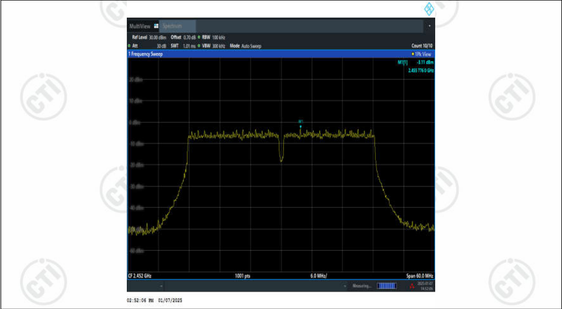
11N40SISO-Ant2-2452-0~Reference-PASS
