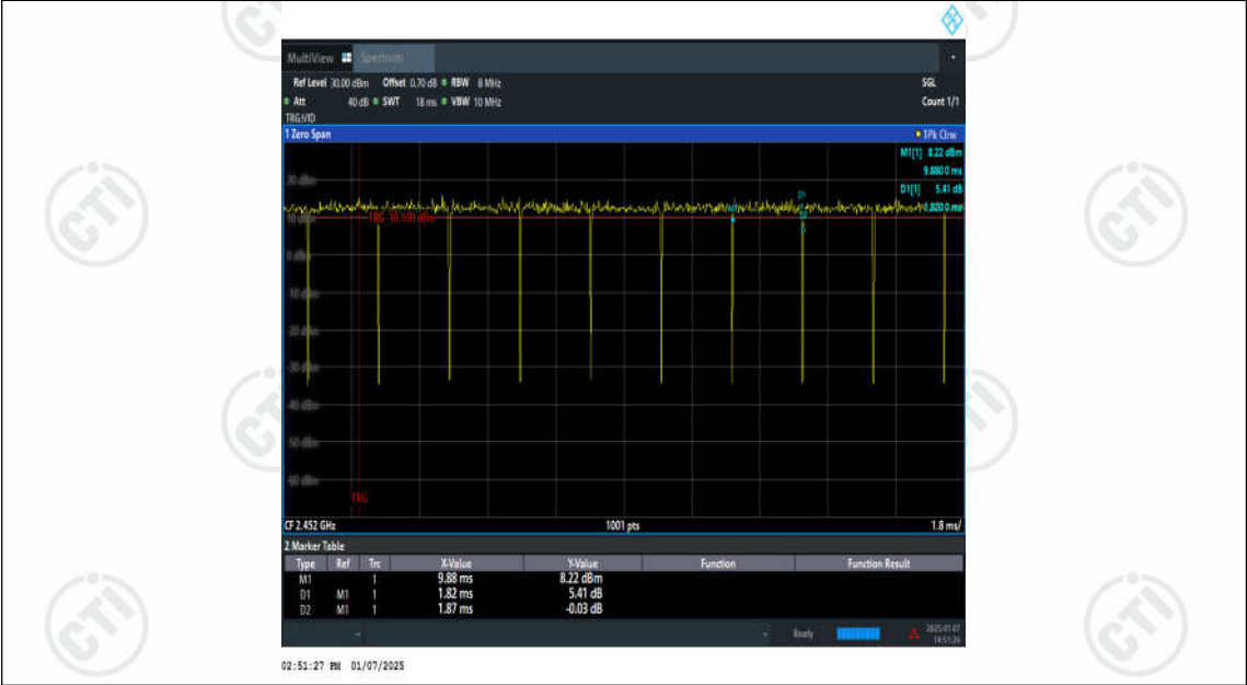
NTNV-11N40SISO-Ant2-2452
