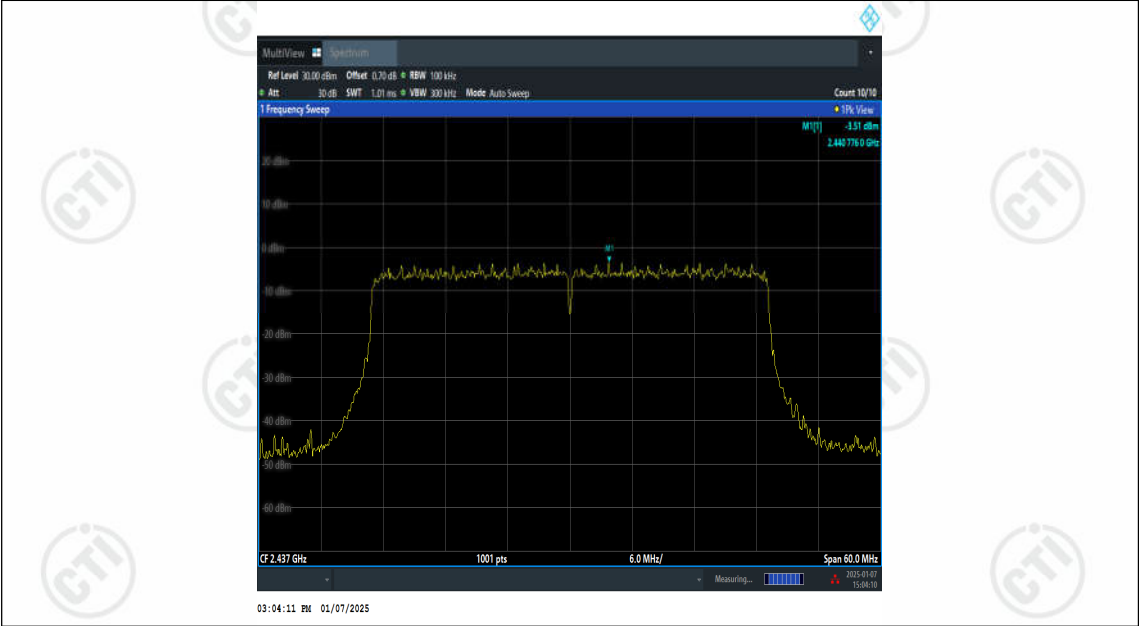
11AX40SISO-Ant2-2437-0~Reference-PASS
