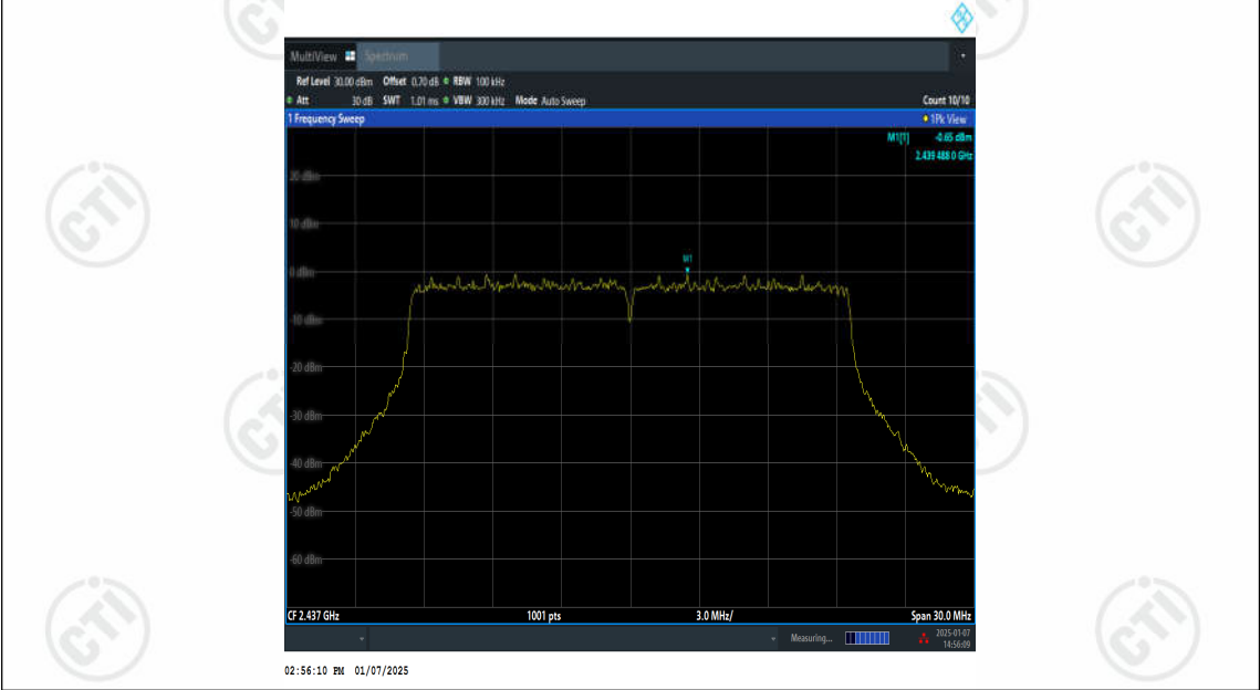
11AX20SISO-Ant2-2437-0~Reference-PASS
