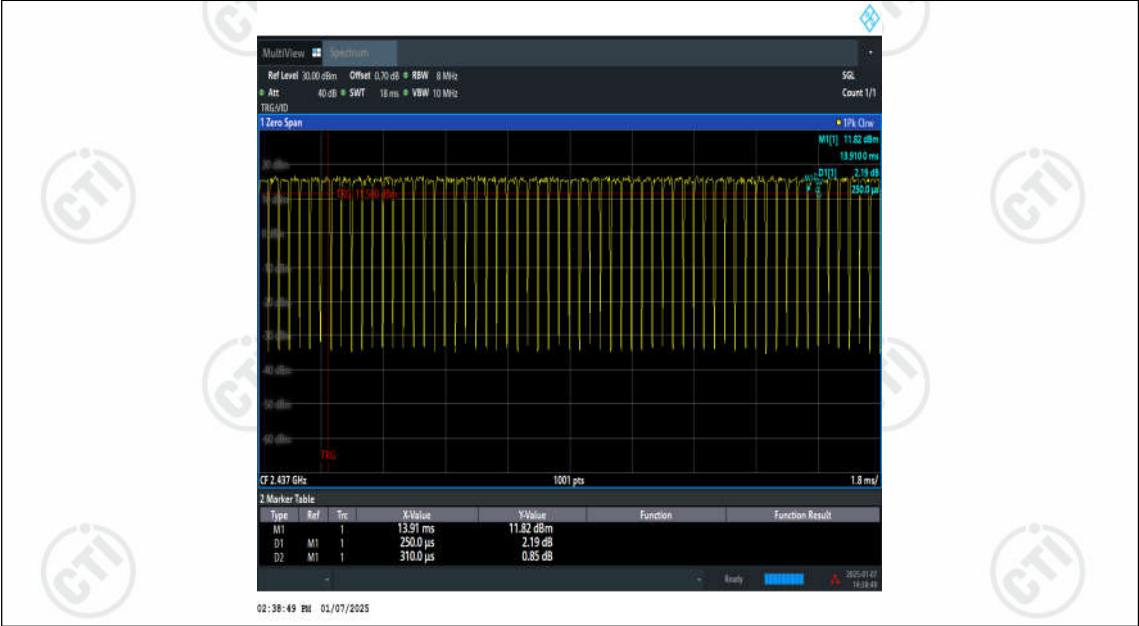
NTNV-11G-Ant2-2437
