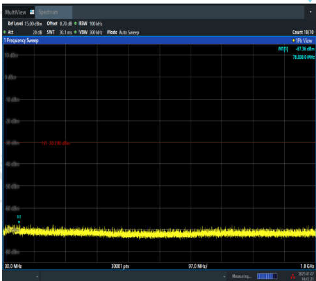
11N20SISO-Ant2-2412-30~1000-PASS
