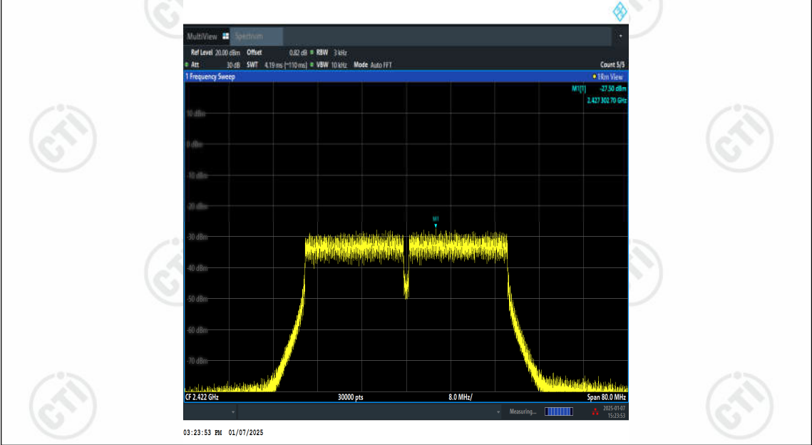
11N40MIMO-Ant2-2422-PASS
