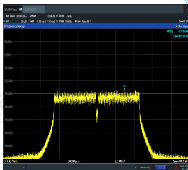
11N40MIMO-Ant2-2437-PASS
