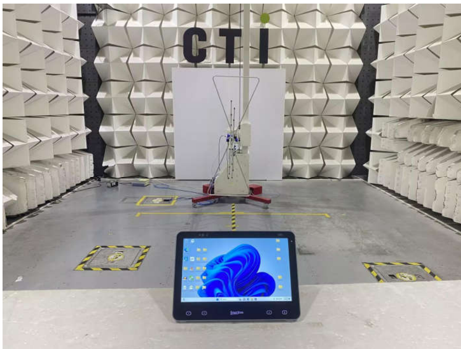
Radiated spurious emission Test Setup-1 (Below 1GHz)close up
