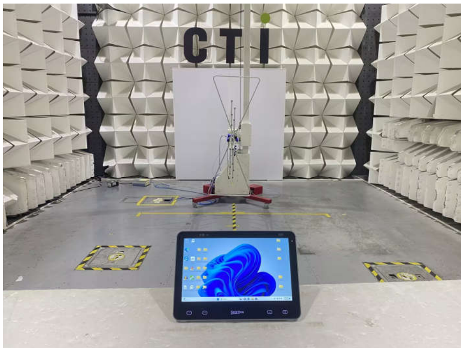
Radiated spurious emission Test Setup-1(with adapter)(Below 1GHz)close up
