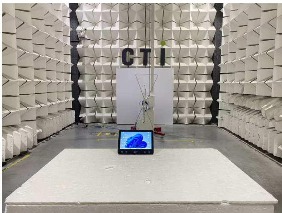
Radiated spurious emission Test Setup-2(without adapter)(Below 1GHz)
