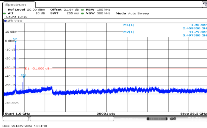
11G_Ant1_2462_1000-26500
