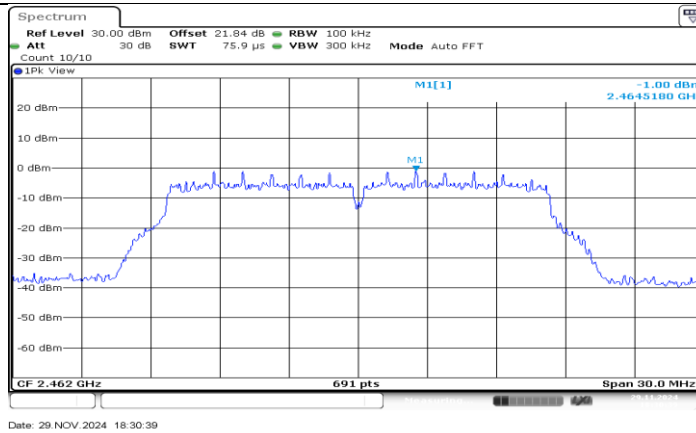
11G_Ant1_2462_0-Reference
