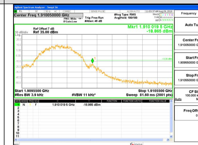
GSM 1900-HCH-GSM
