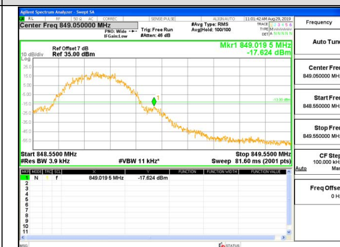
GSM 850-HCH-GPRS
