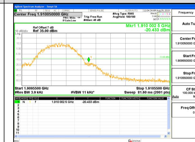
GSM 1900-HCH-GPRS
