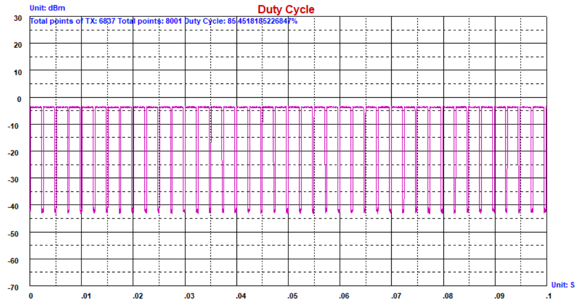
Duty Cycle_BLE_2402_Ant1
