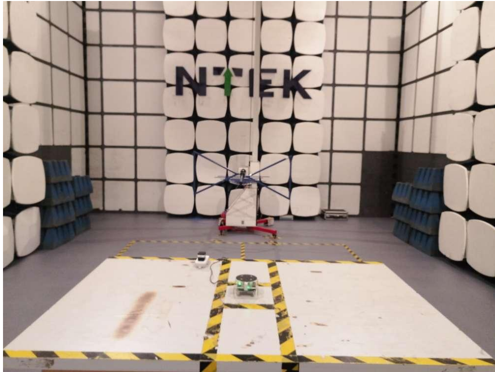
Radiated Measurement Photos (Model: DDKC7Q1)
