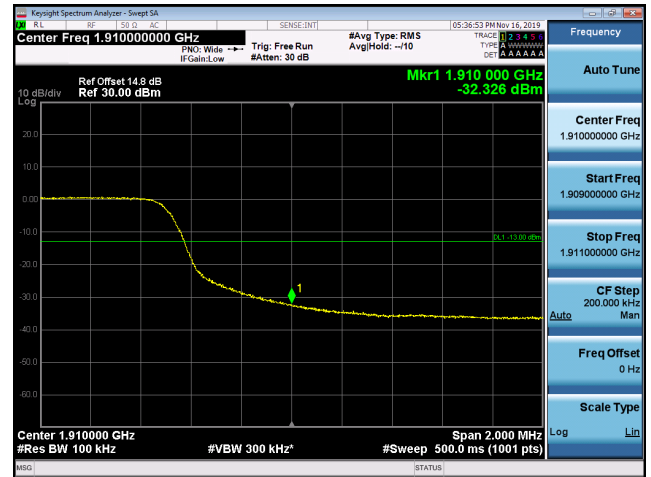
16QAM High channel-50 RB offset 0
