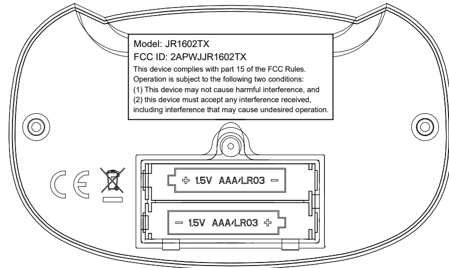
JR1602TX FCC ID Label Location
