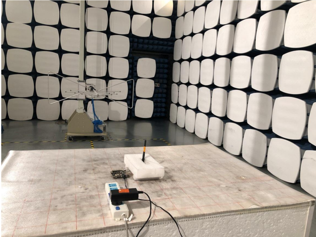
Radiated Spurious Emission Below 1GHz External antenna
