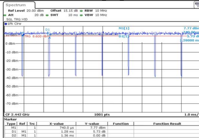
11N20SISO_Ant1_2442
