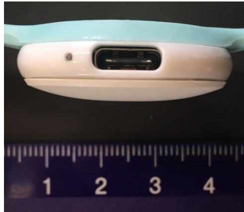
Right Side View – Close Up Sensor Part
