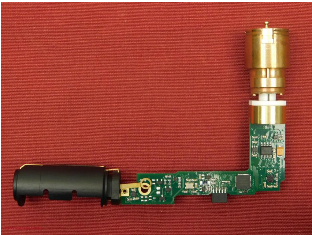
Picture 24: EUT – bottom view without lower half shell
