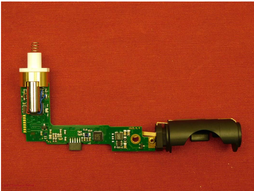
Picture 30: EUT – top view without lock
