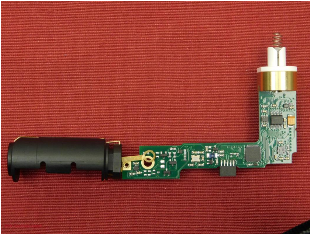
Picture 31: EUT – bottom view without lock
