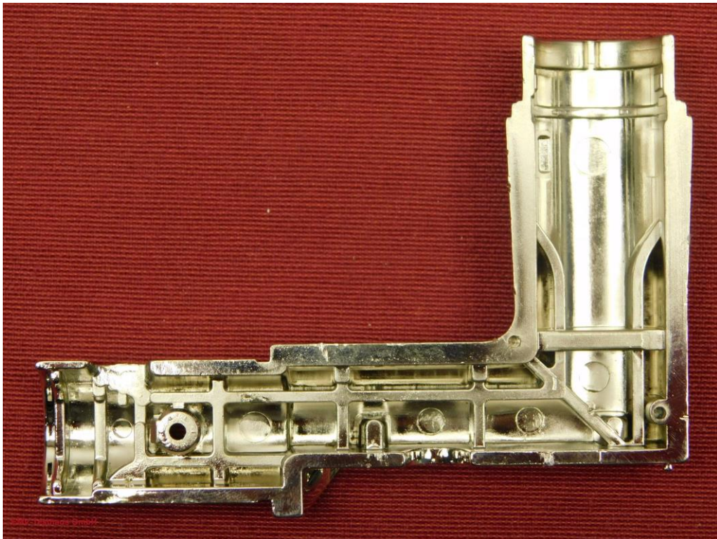
Picture 19: Upper half shell – top view
