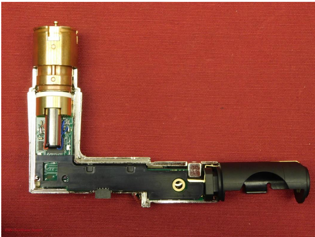
Picture 18: EUT – top view without upper half shell
