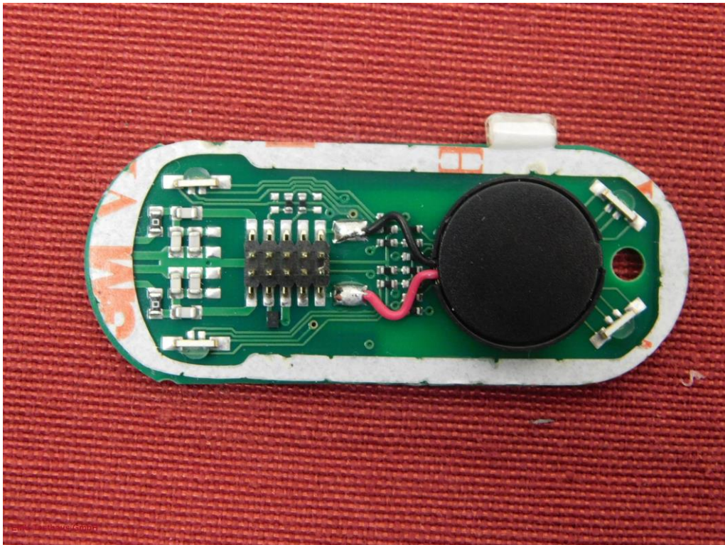
Picture 7: RFID board – bottom view
