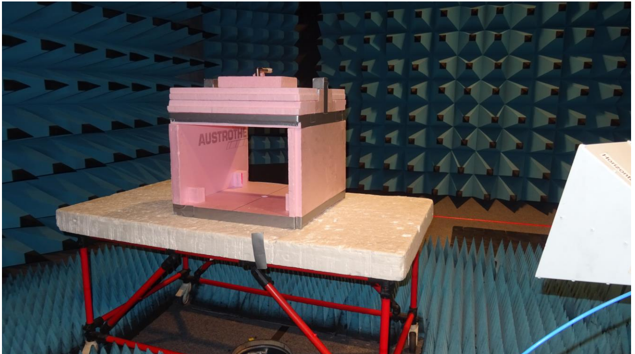
Picture 8: FS-SAC, field strength and band edge measurement (front view)
