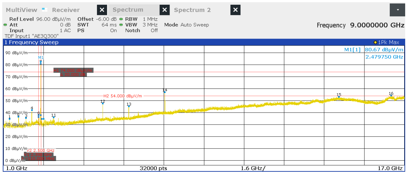
Figure 29: Chart of emissions test from 1 GHz to 17 GHz on highest channel, EUT position Y, antenna polarization vertical
