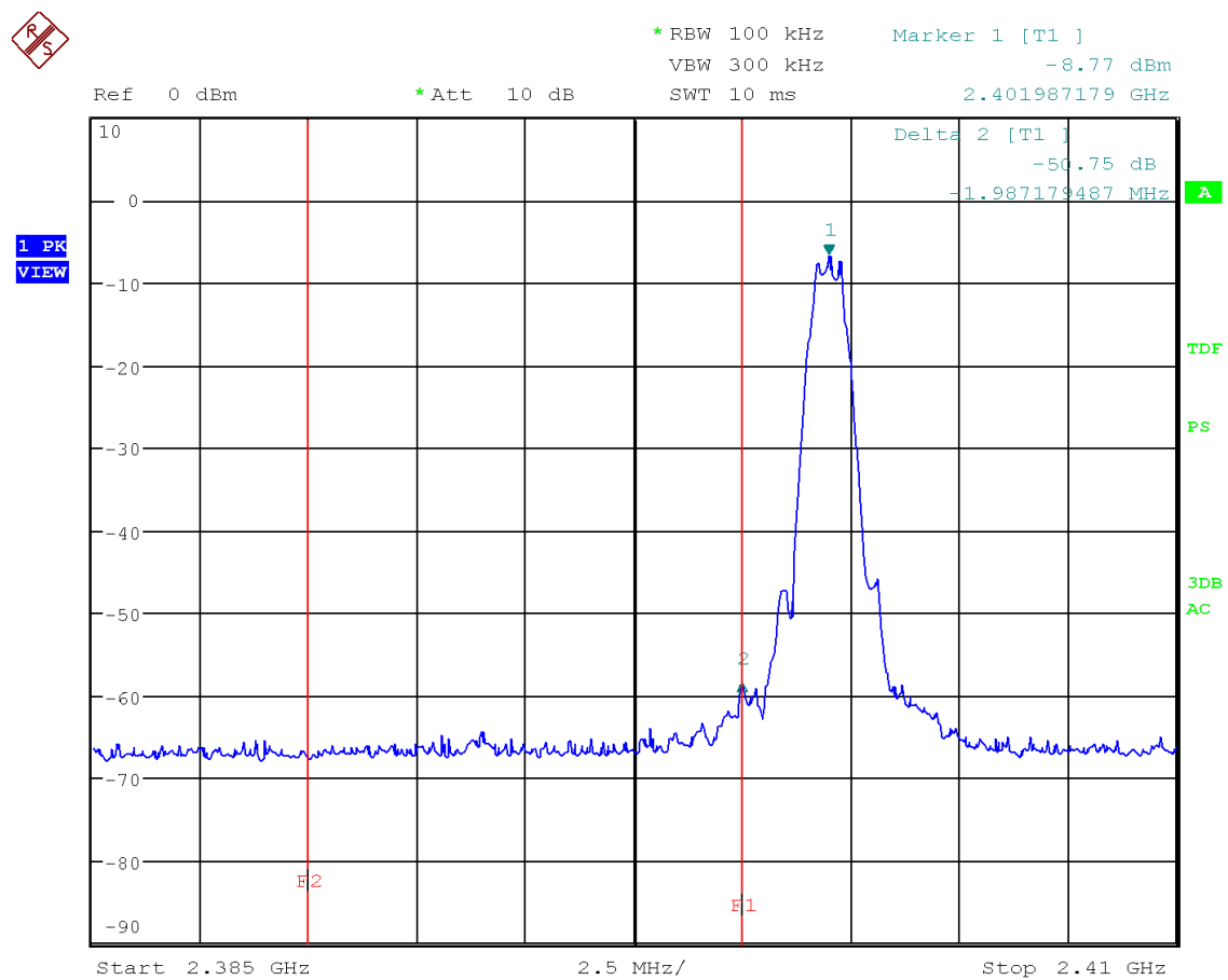
Figure 18: Chart of band-edge measurement on lowest channel
