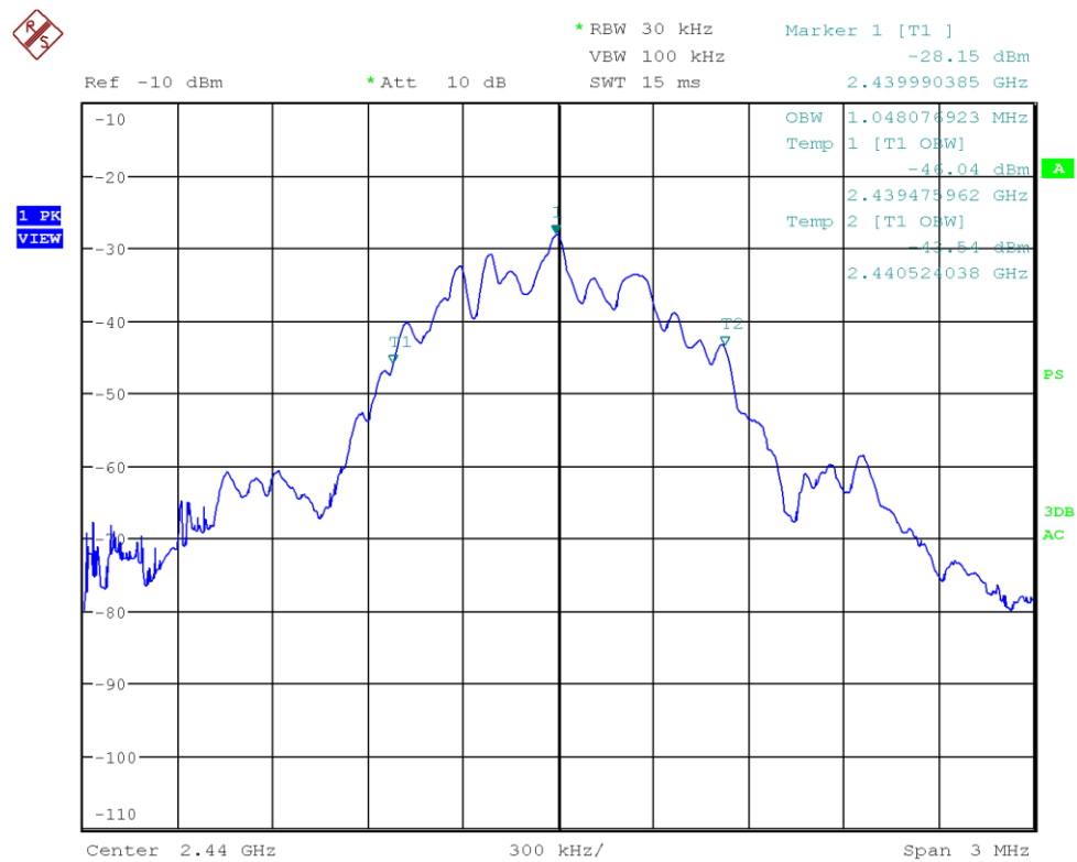
Figure 10: Chart of occupied bandwidth test on middle channel
