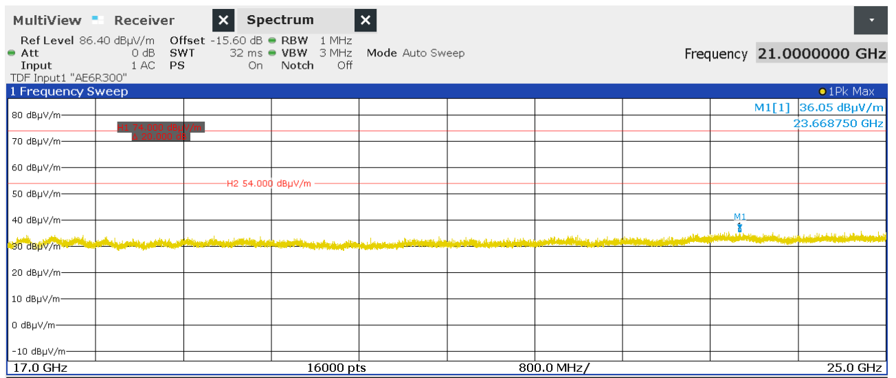
Figure 26: Chart of exploratory radiated emissions measurement from 17 GHz to 25 GHz on lowest channel
