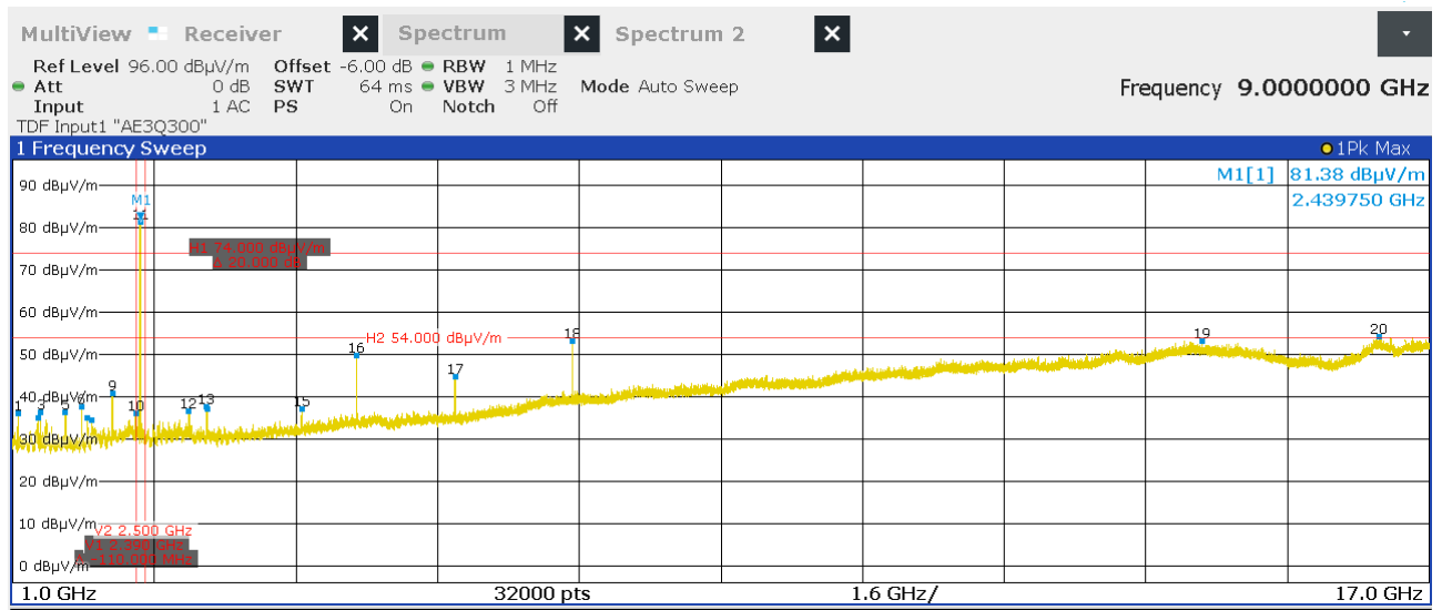
Figure 27: Chart of radiated emissions pre-measurement from 1 GHz to 17 GHz on middle channel, EUT position Y, antenna polarization vertical
