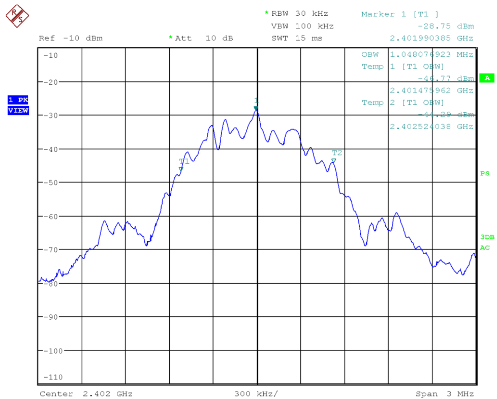
Figure 9: Chart of occupied bandwidth test on lowest channel
