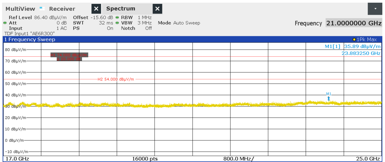
Figure 28: Chart of exploratory emissions measurement from 17 GHz to 25 GHz on middle channel
