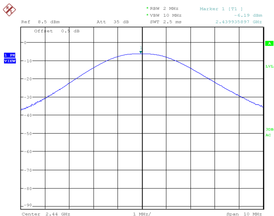
Figure 13: Chart of conducted output power on middle channel
