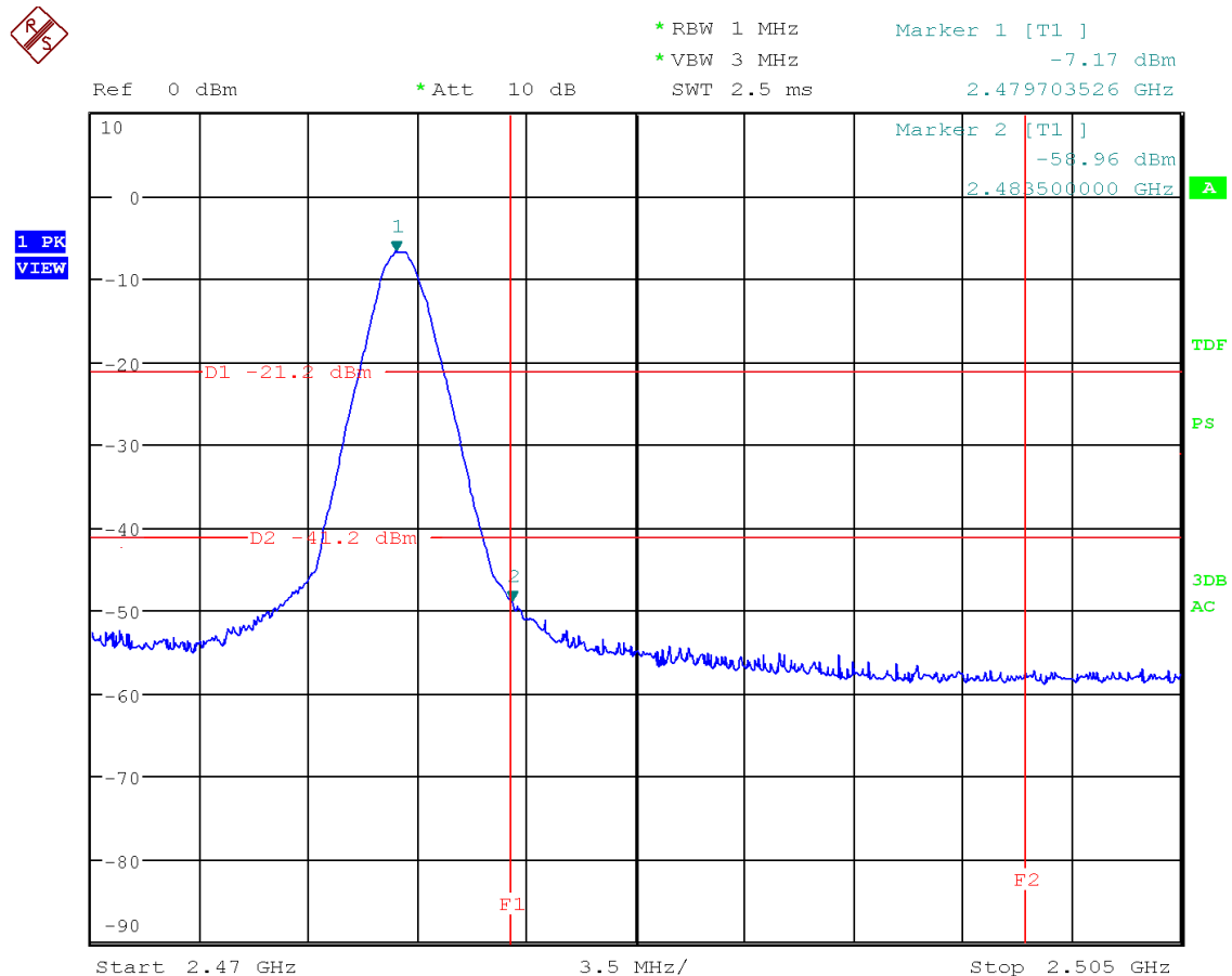
Figure 19: Chart of band-edge measurement on highest channel (PK)
