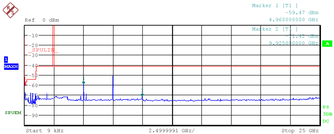
Figure 22: Chart of emissions test from 9 kHz to 25 GHz on highest channel, PK-detector
