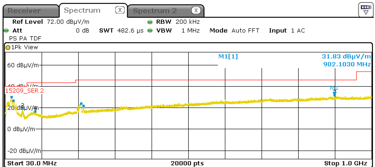
Figure 24: Chart of emissions test from 30 MHz to 1 GHz on lowest channel, EUT position Y, antenna polarization vertical
