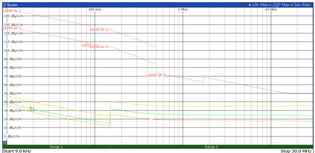
Figure 23: Chart of emissions test below 30 MHz on lowest channel, EUT position Z, antenna parallel to the EUT
