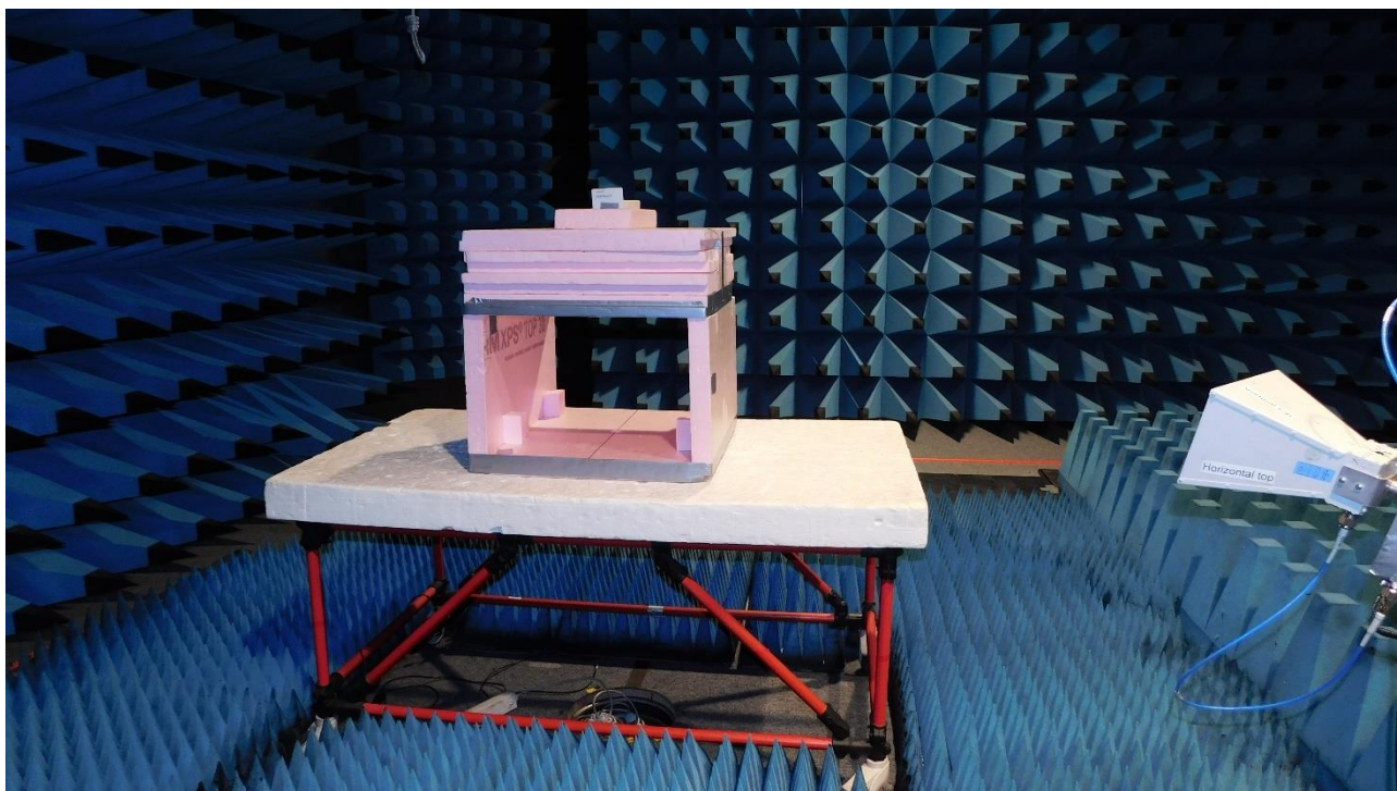
Picture 5: FS-SAC, radiated emission test 1 GHz – 17 GHz (front view)
