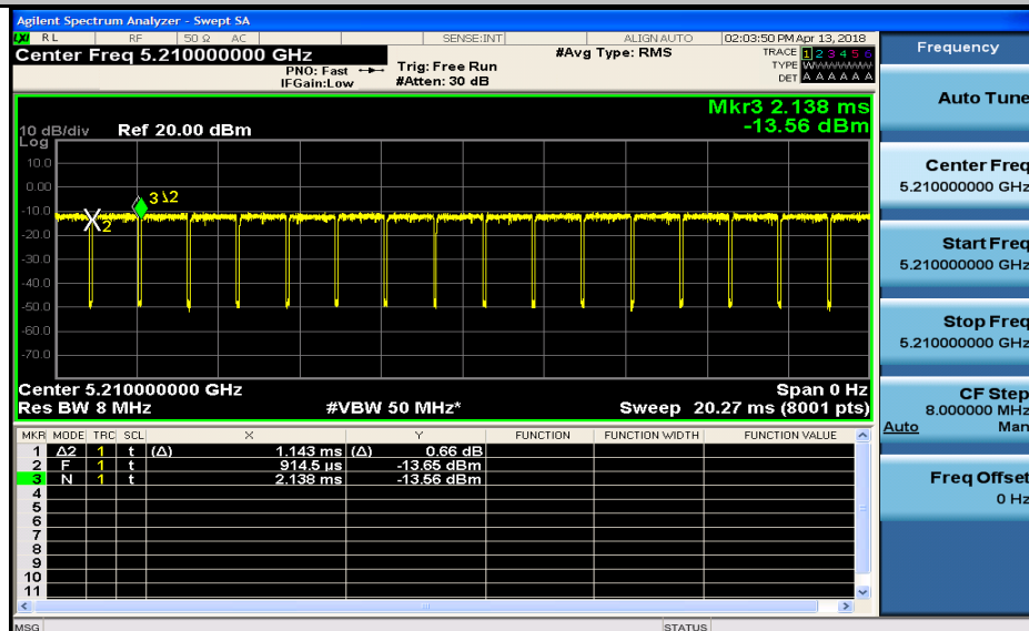
Duty Cycle_11AC80_5210_ANT4
