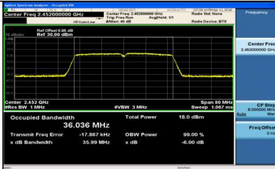
Occupied Bandwidth_11N40SISO_2452_Ant1
