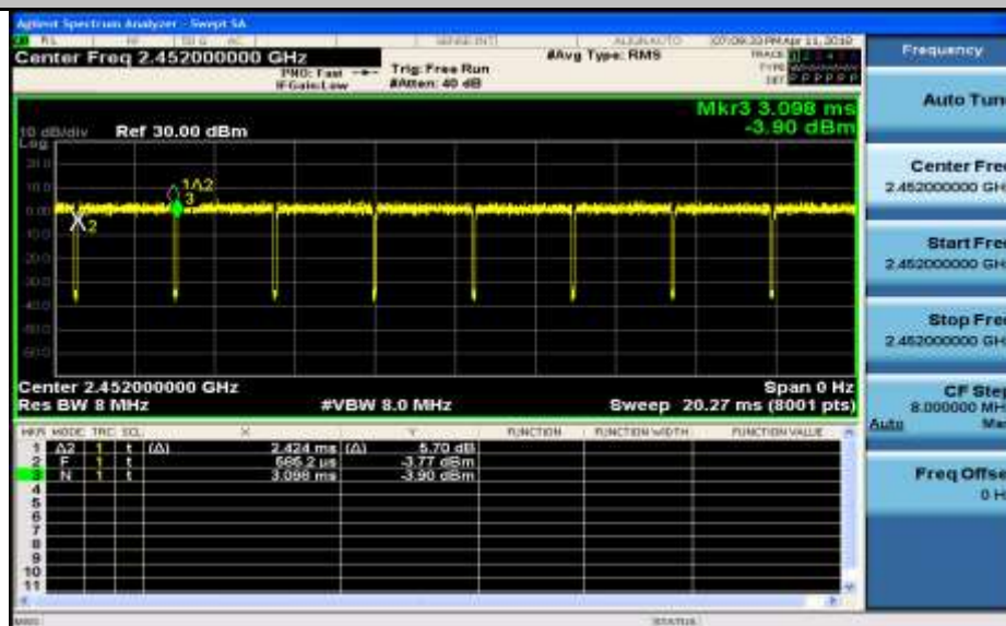
Duty Cycle_11N40SISO_2452_Ant1
