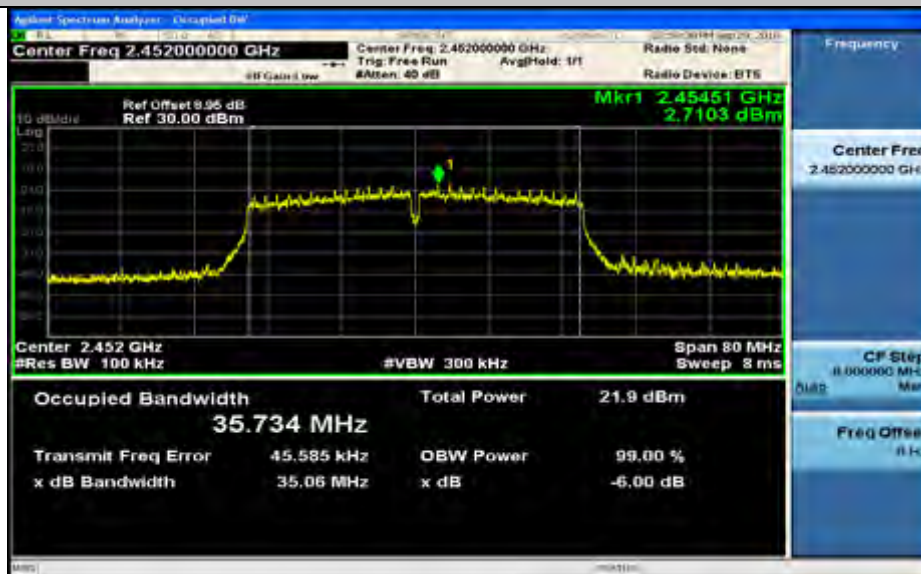
6dB Bandwidth_11N40SISO_2452_Ant2
