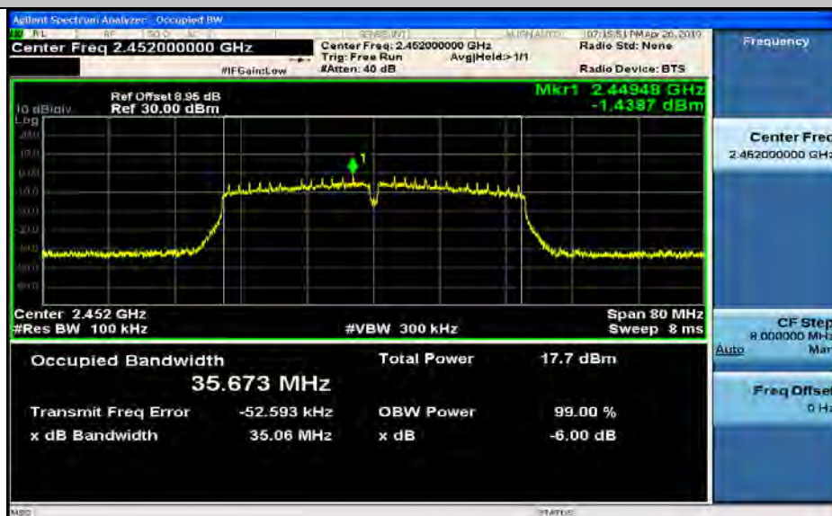
6dB Bandwidth_11N40SISO_2452_Ant2
