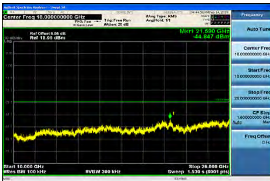
RF Conducted Spurious Emissions_11N20SISO_2412
