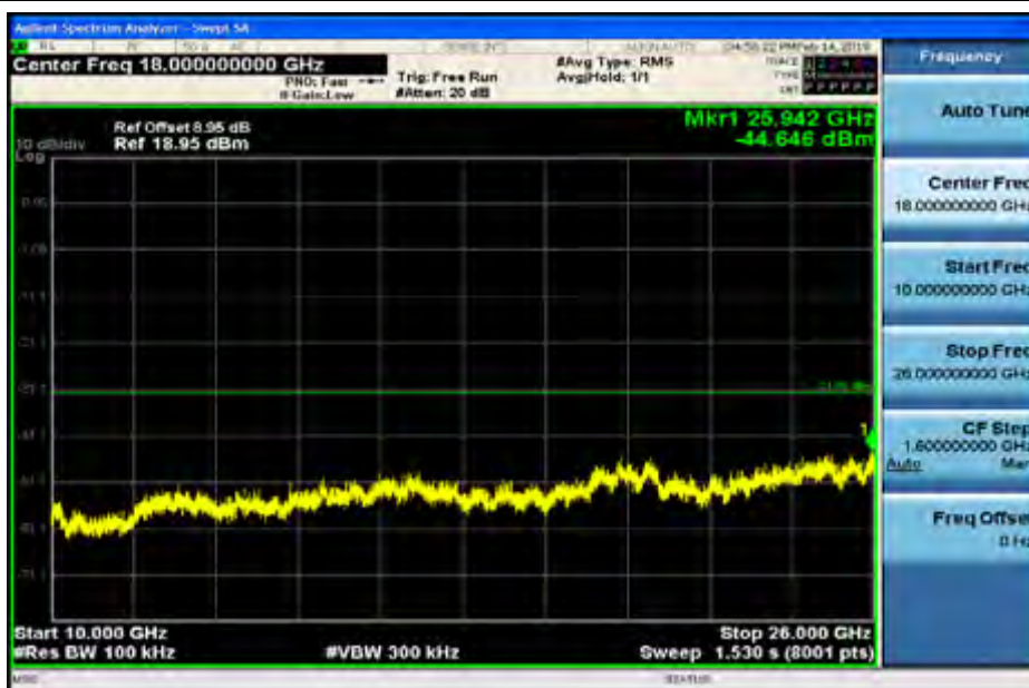
RF Conducted Spurious Emissions_11N20SISO_2462
