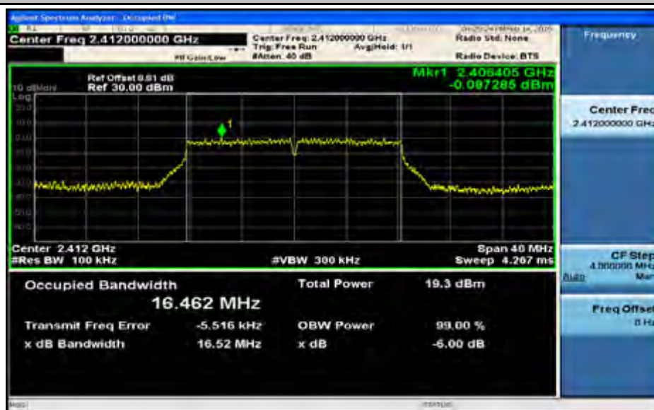
6dB Bandwidth_11G_2437_Ant1
