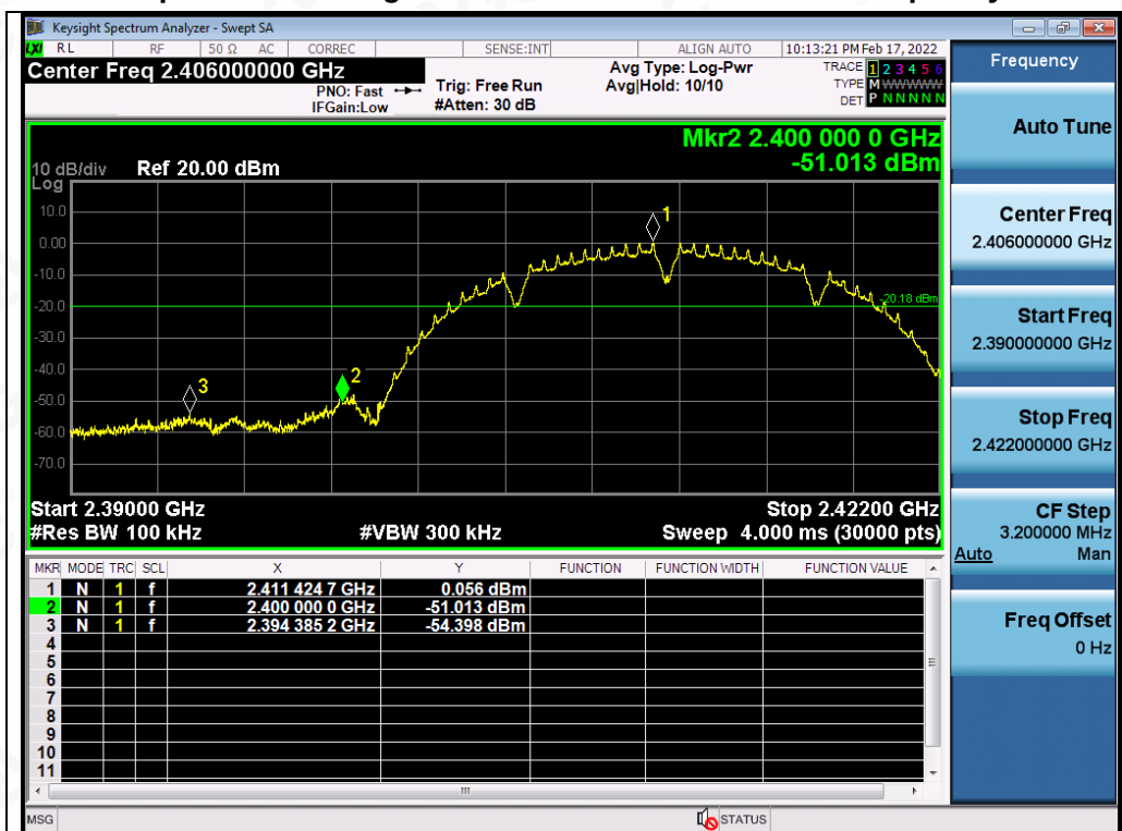
Test Graph 802.11b ANT1 2412 1Mbps Lower Band Edge Emissions
