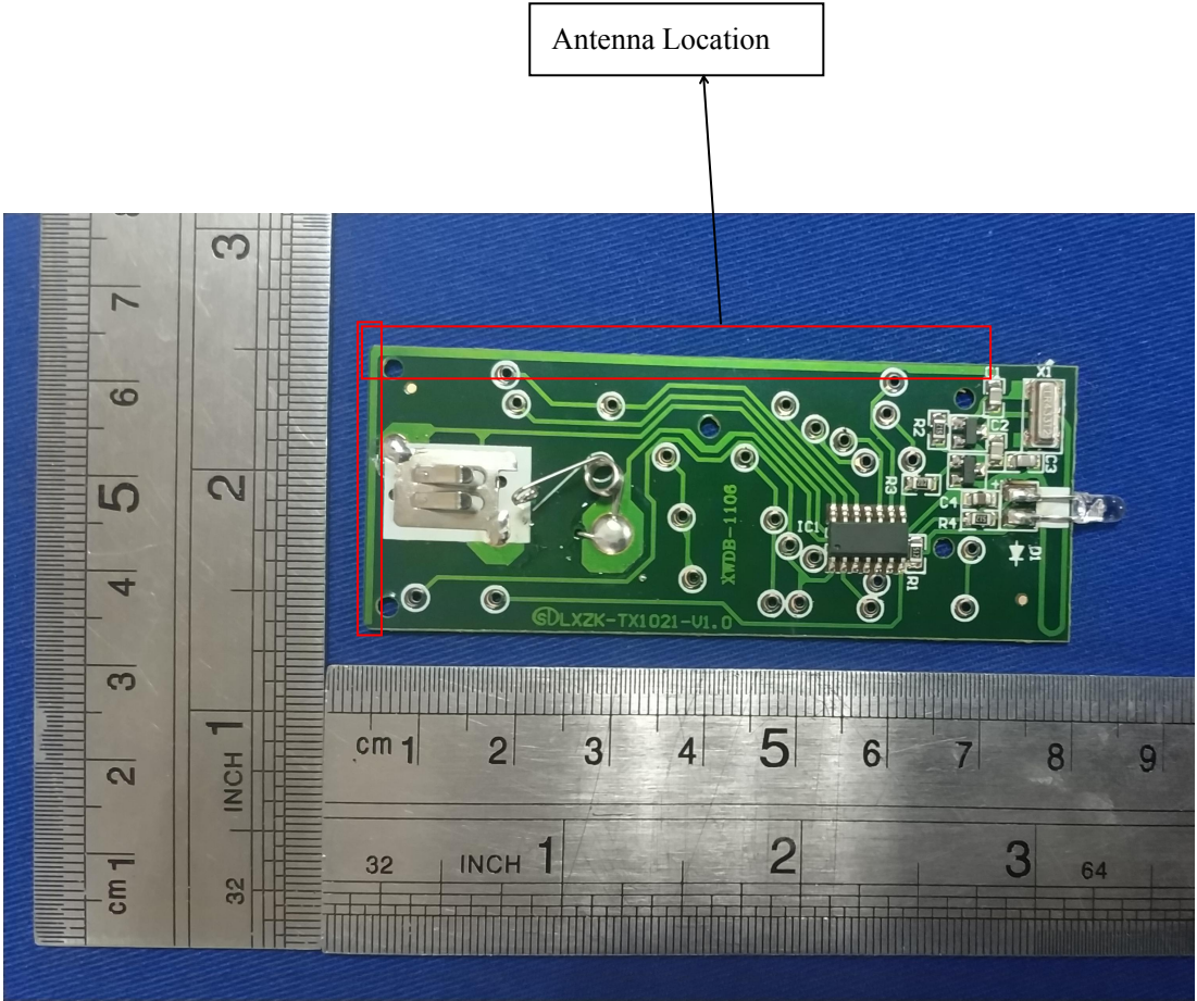
EUT – PCB View
