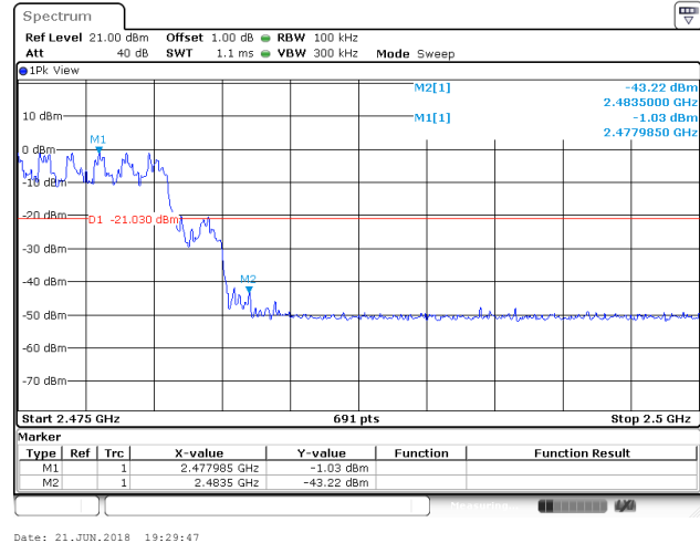
8-DPSK: Band Edge-High Channel (Hopping Mode)
