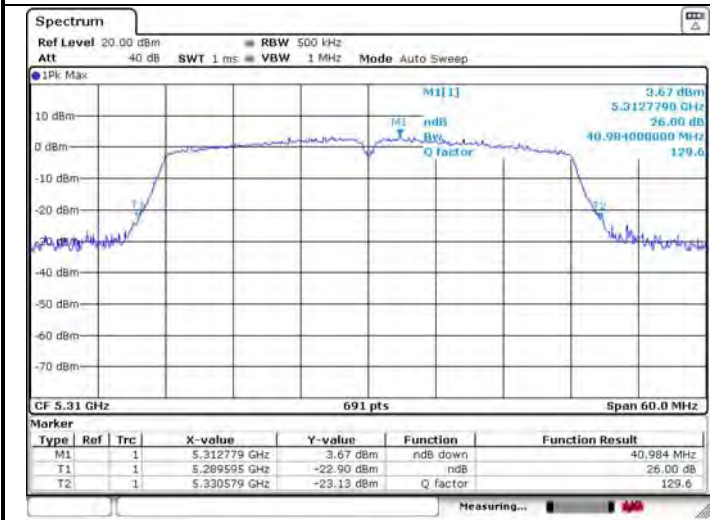
26dB Bandwidth
