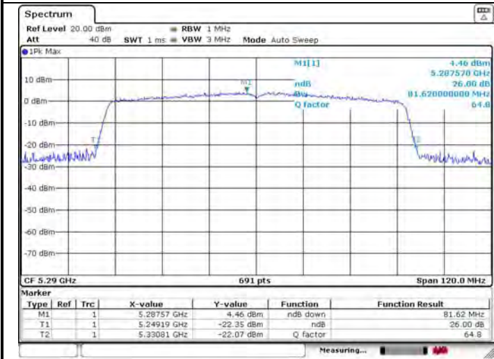
26dB Bandwidth
