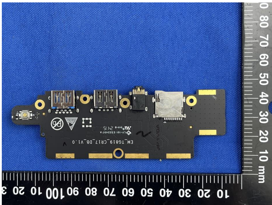
SECONDARY BOARD 2 REAR VIEW (WITHOUT SHIELDING)
