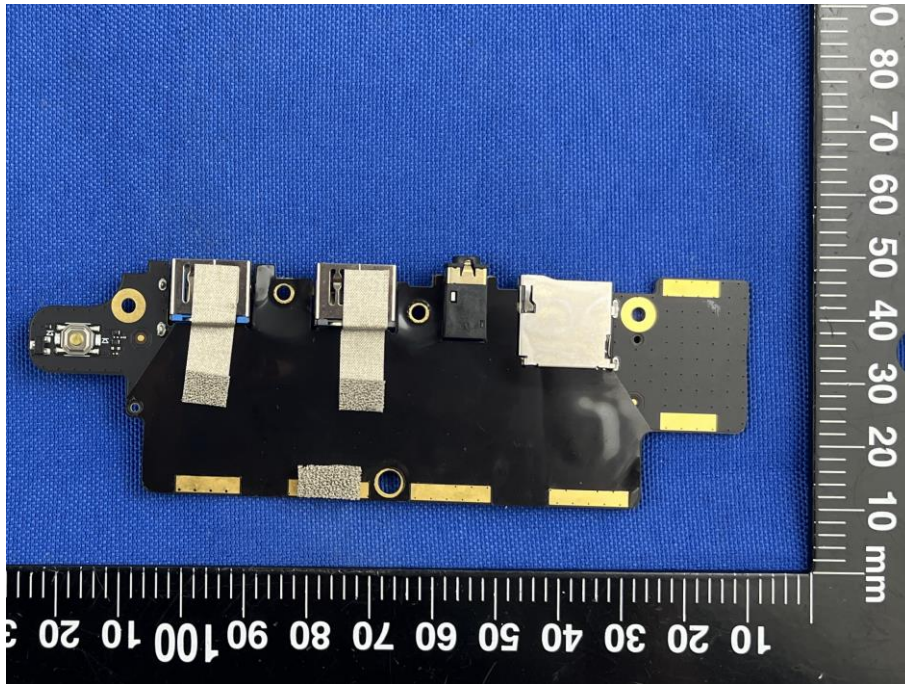
SECONDARY BOARD 2 REAR VIEW (WITH SHIELDING)
