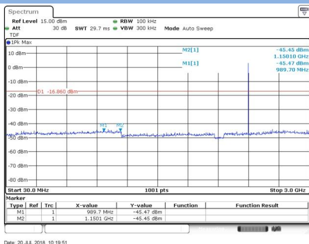
GFSK (BLE) LOW CHANNEL , SPURIOUS 30 MHz ~ 3 GHz
