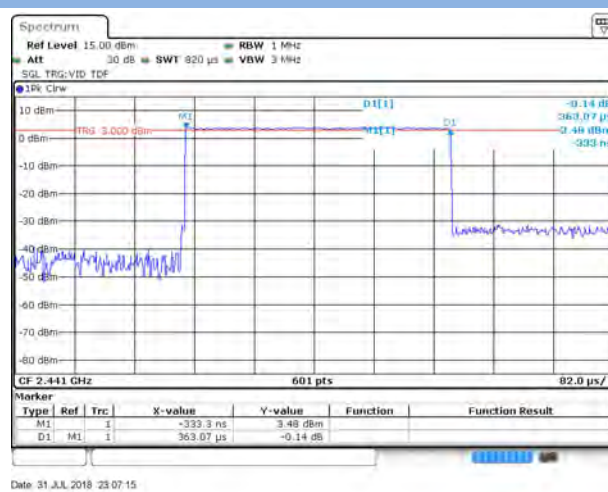
GFSK DH1
