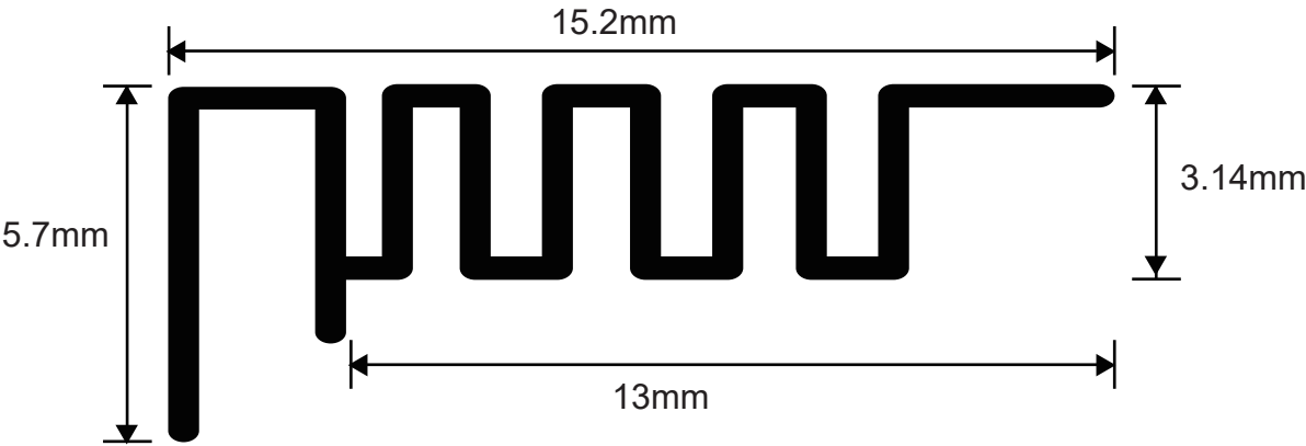
Antenna Photo & Length (mm)
