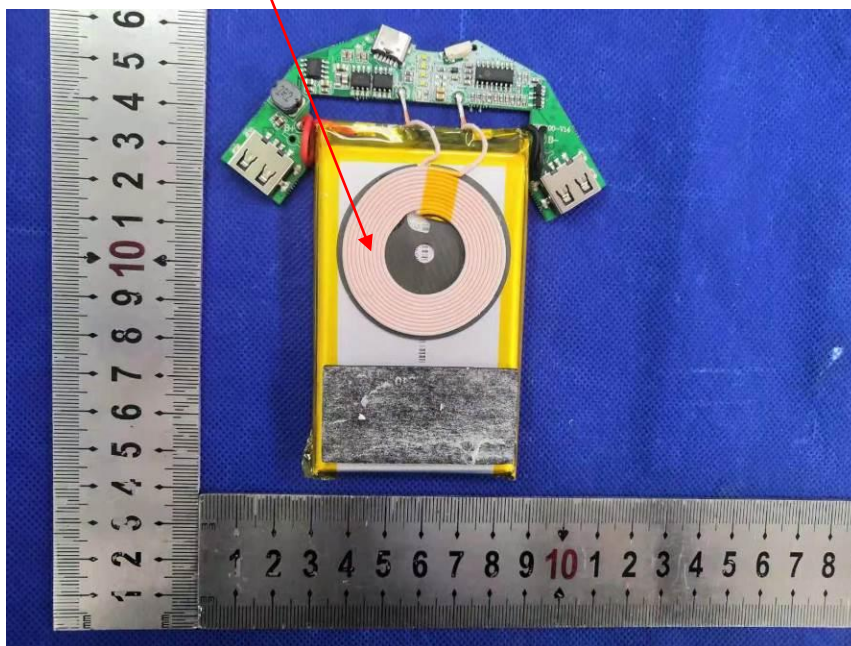
Coil Antenna
