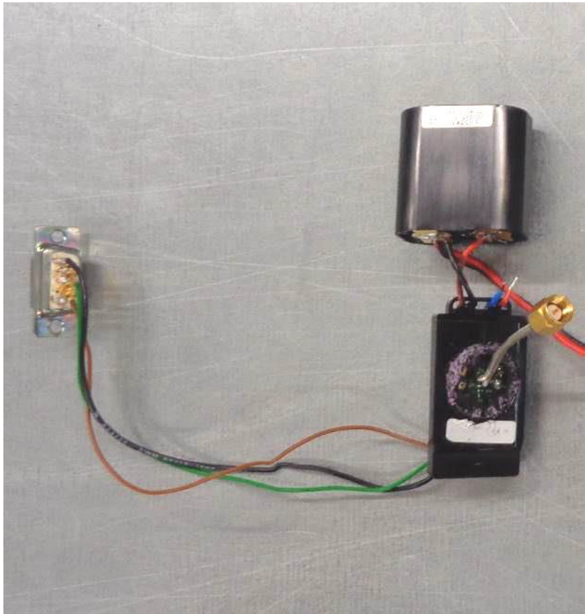
RF module (Prototype 2) with temporary antenna connector
