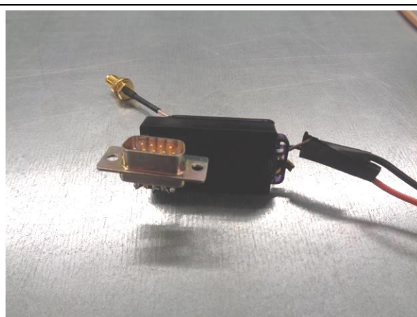
RF module (S/N 220) with temporary antenna connector (rear view)
