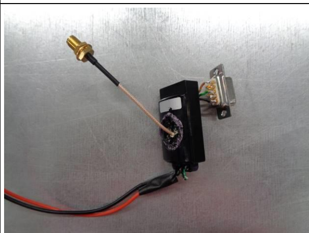
RF module (S/N 220) with temporary antenna connector (front view)
