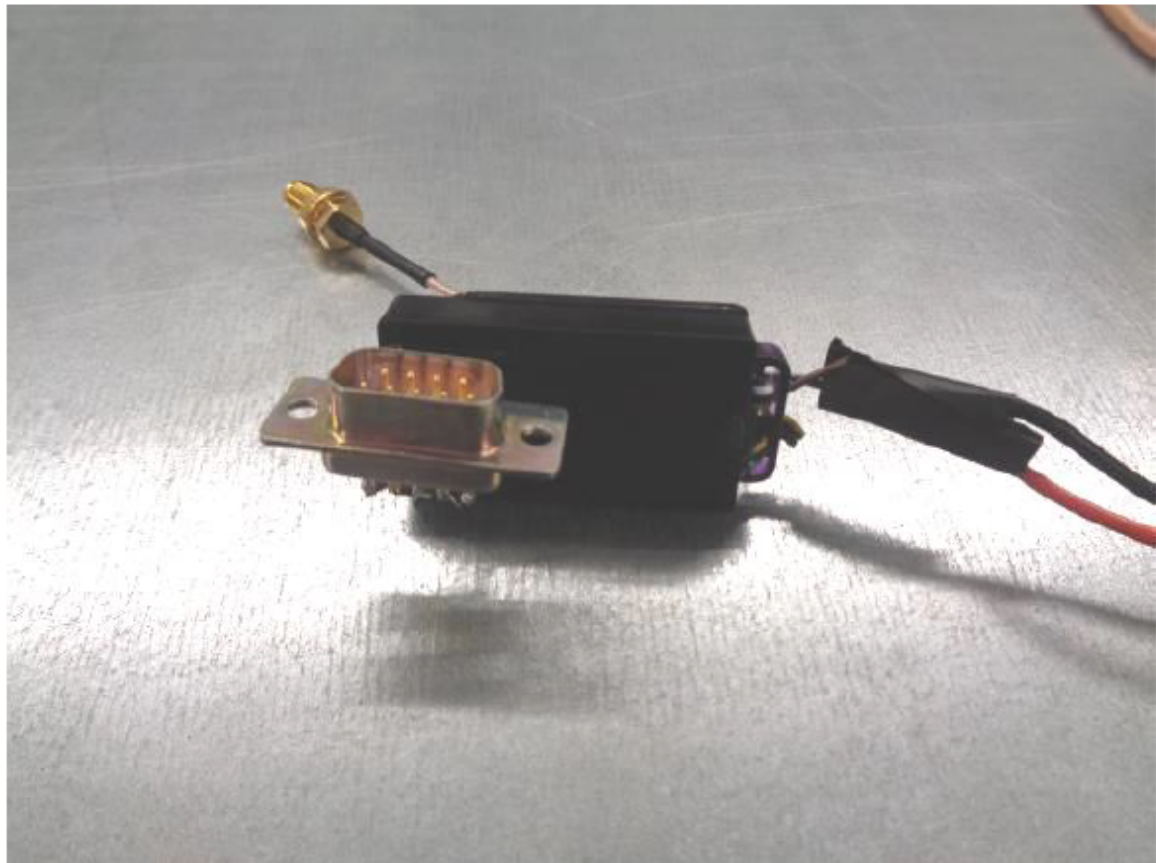
RF module (Prototype 2) with temporary antenna connector (rear view)
