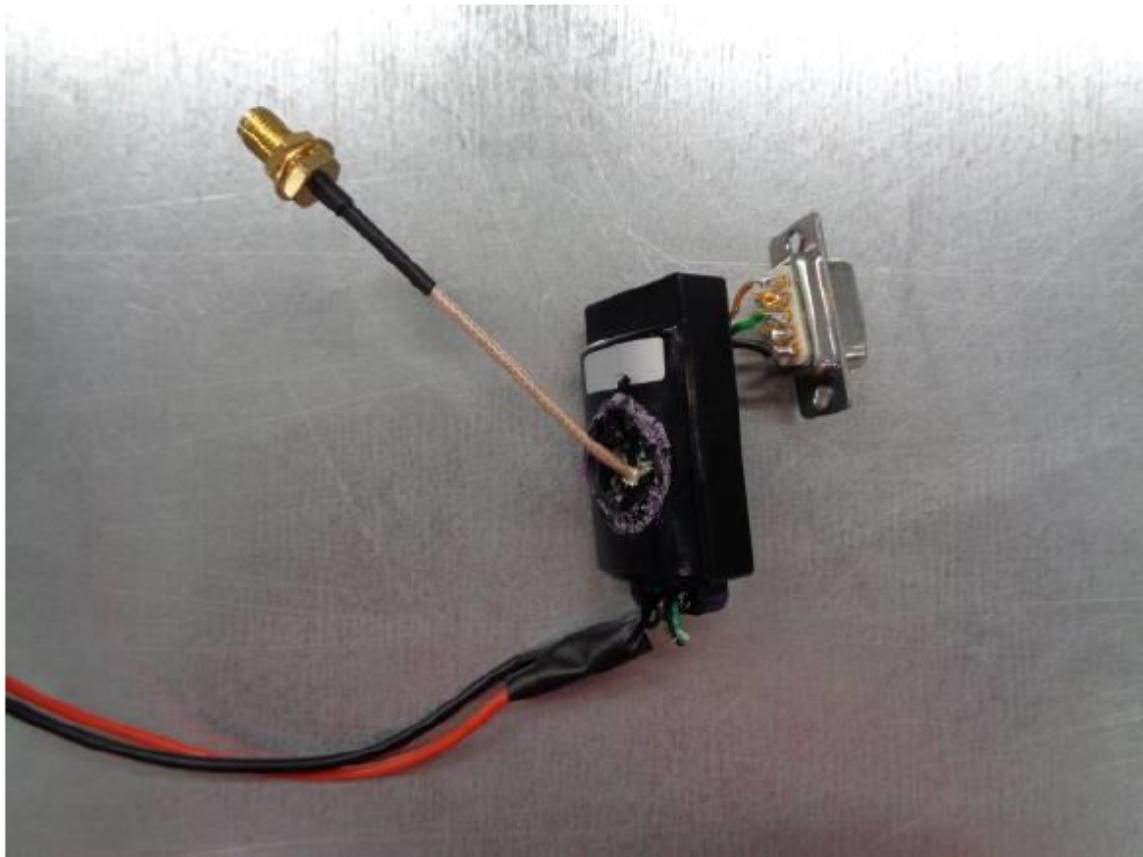
RF module (Prototype 2) with temporary antenna connector (front view)
