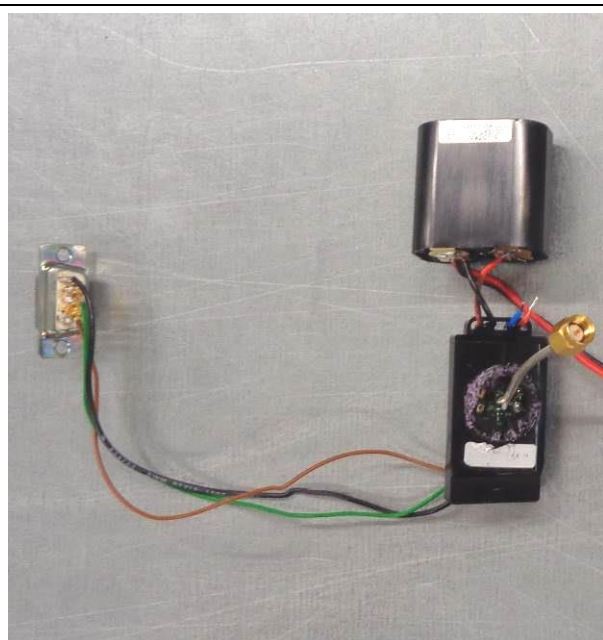
RF module (S/N 222) with temporary antenna connector (top view)
