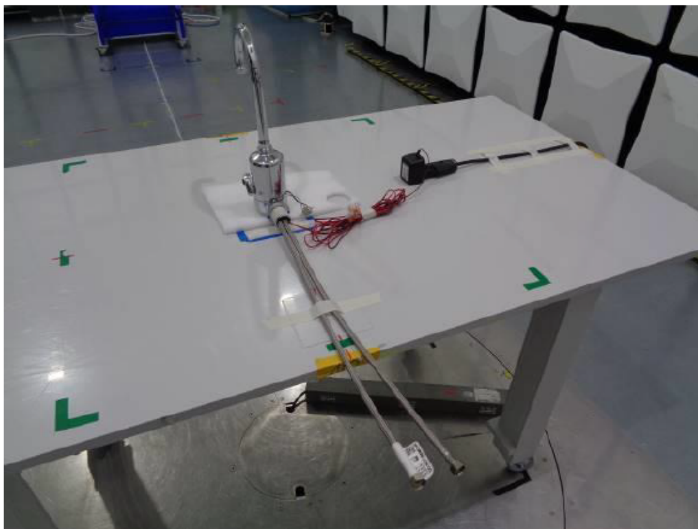
Complete EUT (Prototype 1, rear-top view)
