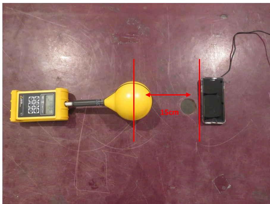
TestPosition B-Exposure photo from side edge surface-Left
