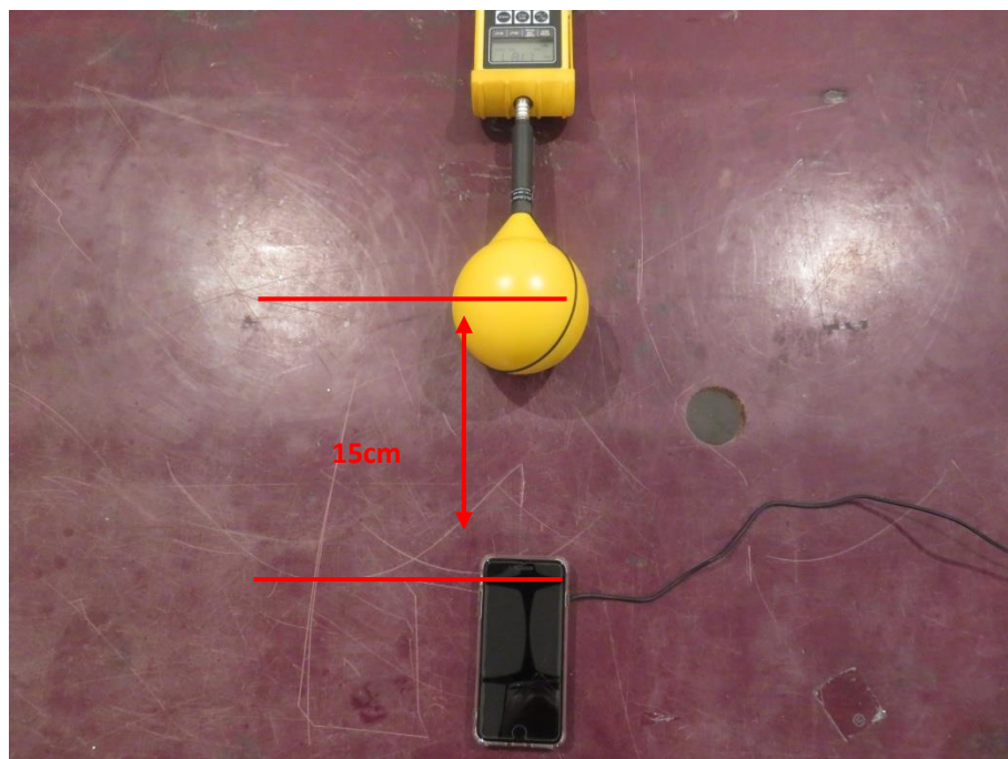
TestPosition A-Exposure photo from side edge surface-Rear
