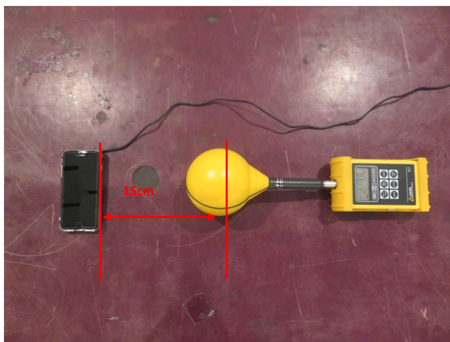
TestPosition D-Exposure photo from side edge surface-Right
