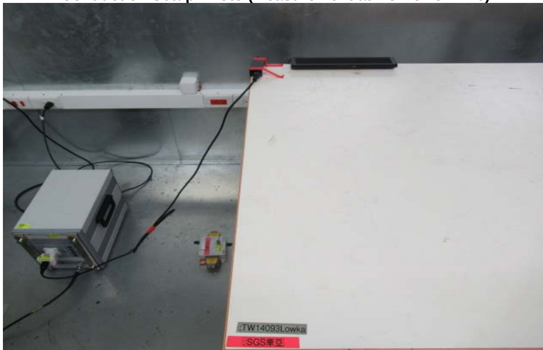
Conduction Setup Photo (Measurement at AC Power Line)
