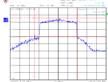
26 dB Bandwidth
