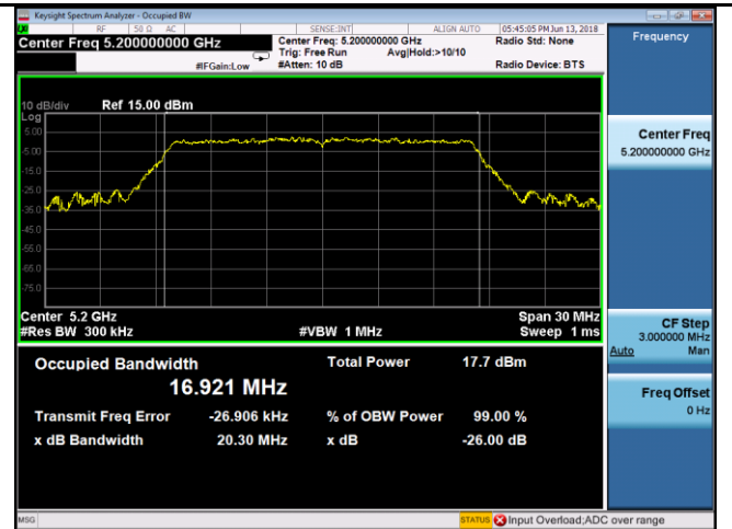
5150-5250MHz Bandwidth - Middle CH 5200
