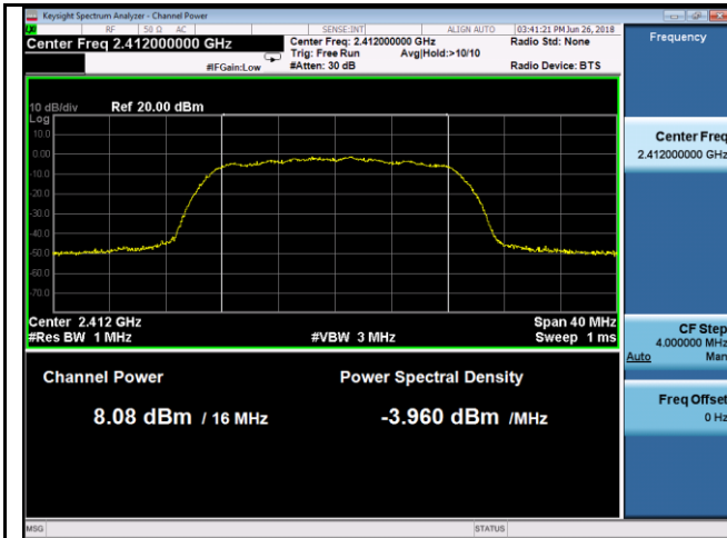
802.11n20 - PK Output power - Low CH 2412
