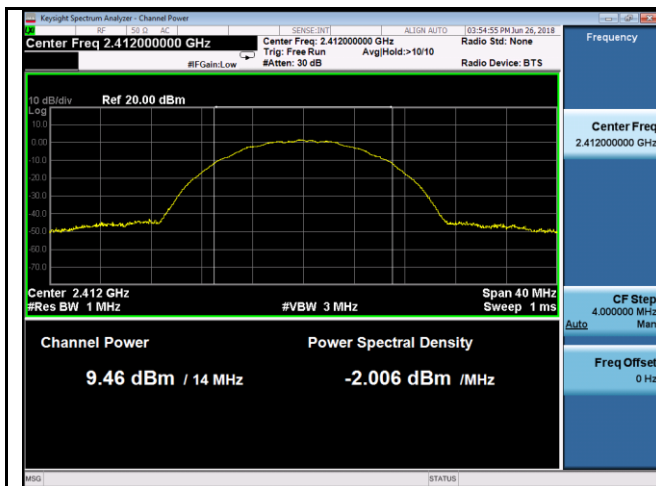
802.11b - PK Output power - Low CH 2412
