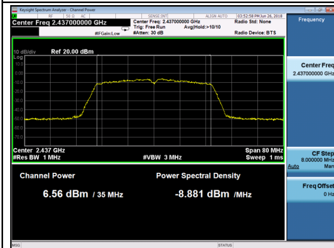
802.11n40 - PK Output power - Mid CH 2437
