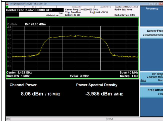
802.11n20 - PK Output power - High CH 2462
