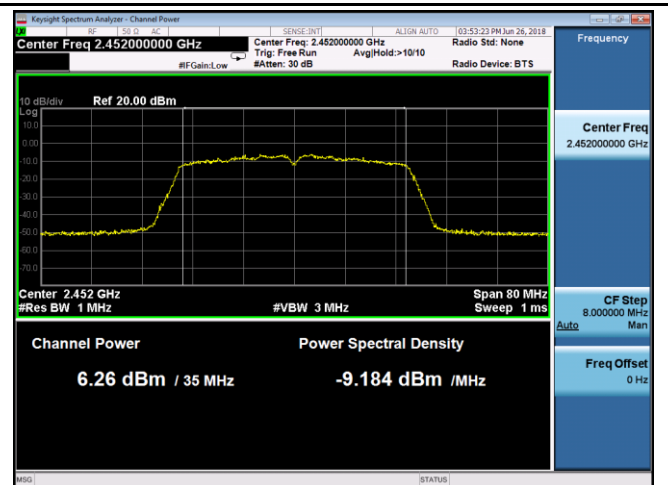
802.11n40 - PK Output power - High CH 2452
