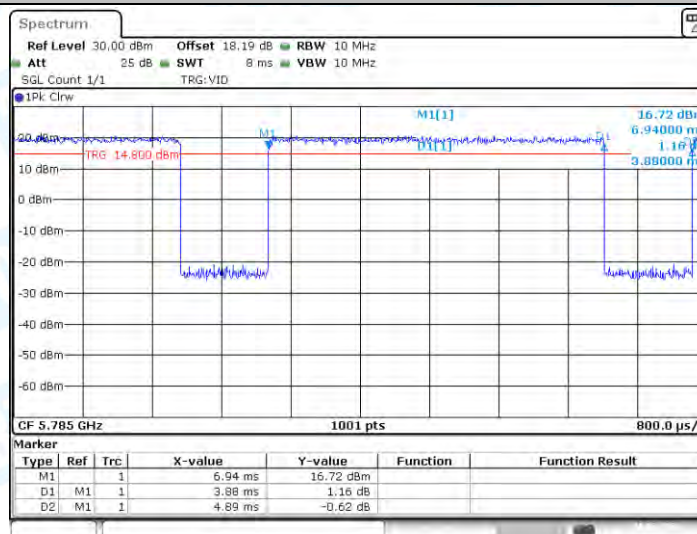
11AX20SISO_Ant1_5785
