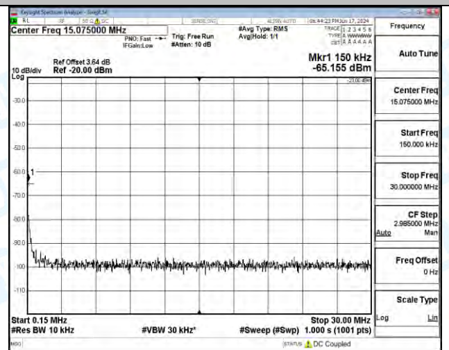
Band12_3MHz_QPSK_23025_15RB#0_1000~3000_1000~3000
