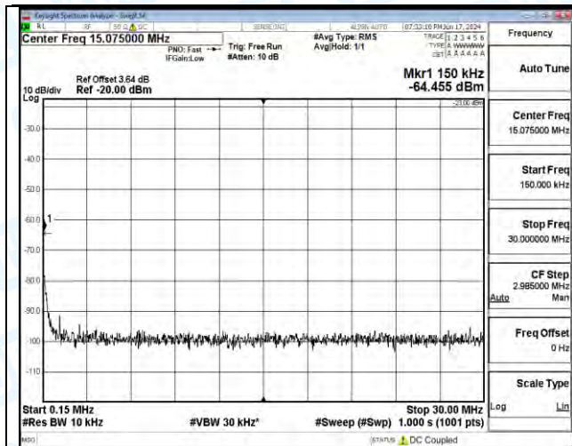
Band12_5MHz_QPSK_23155_1RB#24_1000~3000_1000~3000
