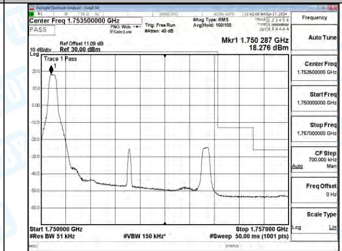
Band4_5MHz_QPSK_20375_25RB#0
