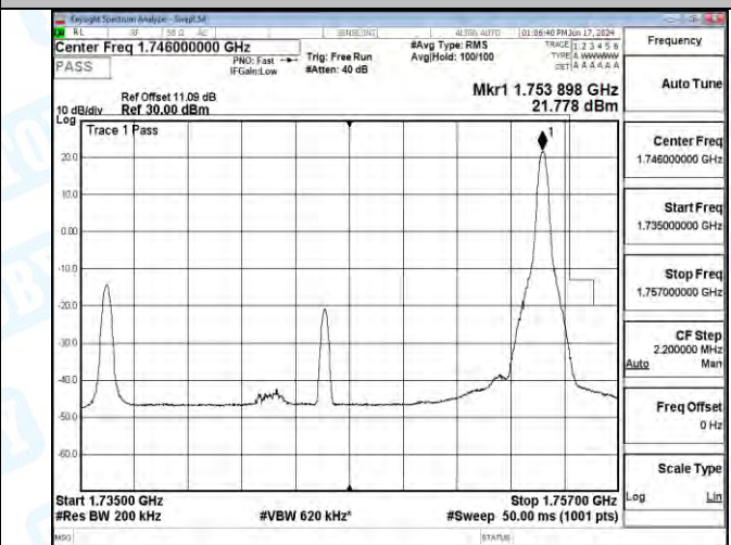
Band4_20MHz_16QAM_20300_1RB#99
