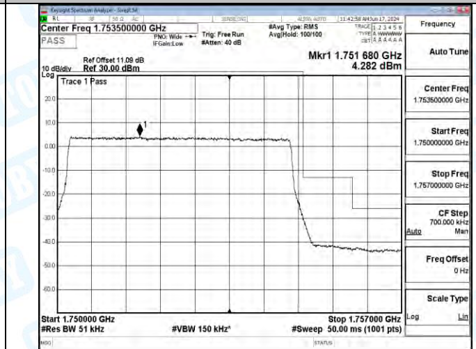
Band4_5MHz_16QAM_19975_1RB#24
