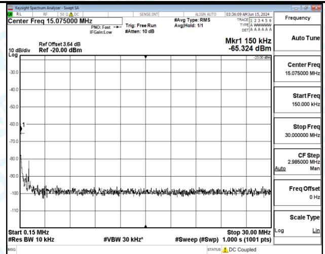
Band5_3MHz_QPSK_20635_1RB#0_1000~3000_1000~3000
